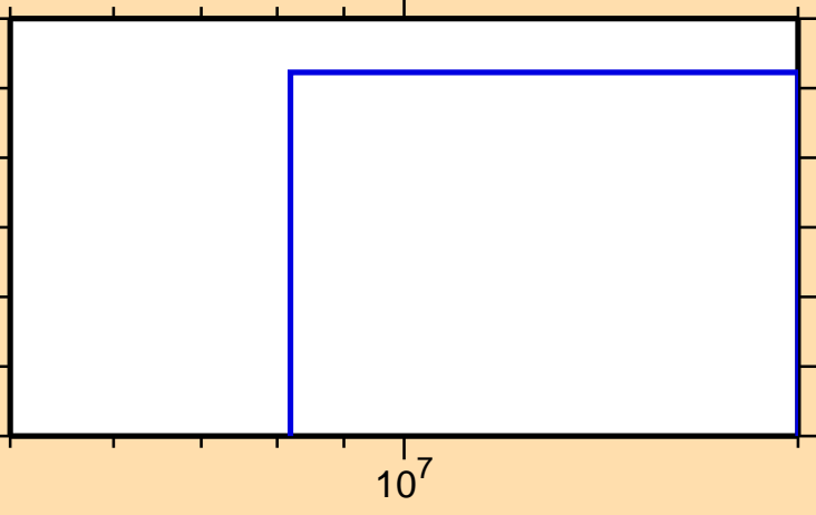
\sigma vs. E for ^{194}\text{Ir}(n,3n)
