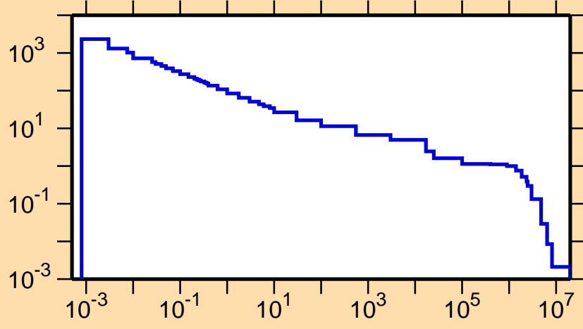
\sigma vs. E for ^{194}\text{Ir}(n,\gamma)
