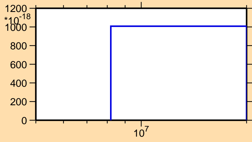
\sigma vs. E for ^{194}\text{Ir}(n,3n\alpha)
