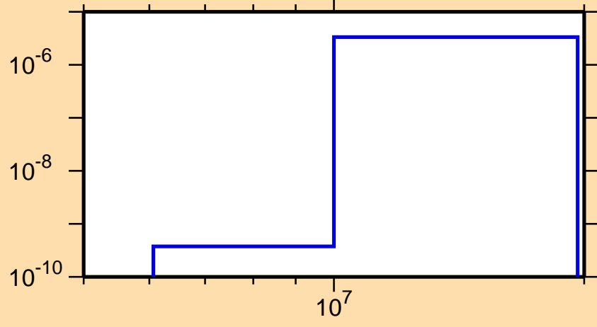
\sigma vs. E for ^{195}\text{Ir}(n,n\alpha)
