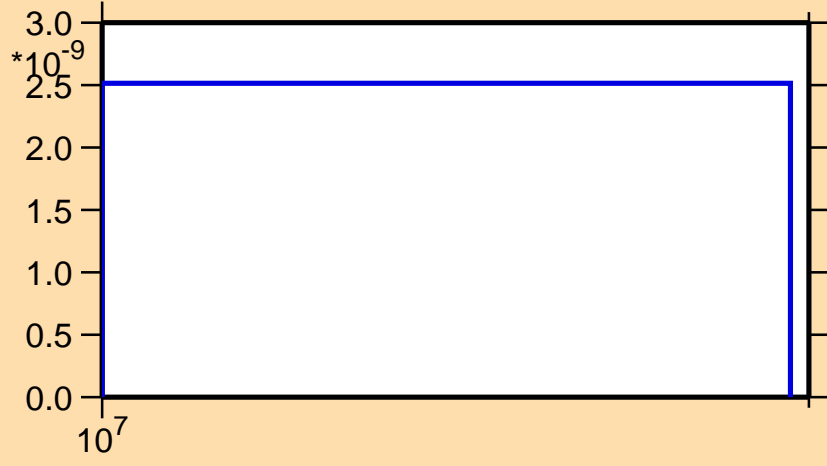
\sigma vs. E for ^{195}\text{Ir}(n,\text{nd})
