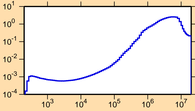
\sigma vs. E for ^{195}\text{Ir}(n,\text{inel.})
