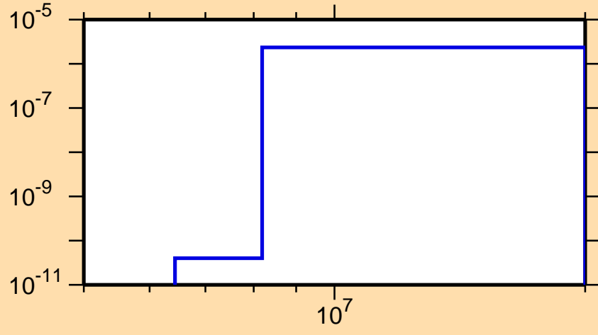
\sigma vs. E for ^{195}\text{Ir}(n,\alpha)
