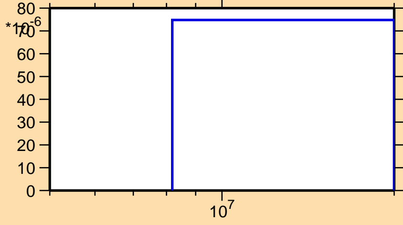
\sigma vs. E for ^{195}\text{Ir}(n,d)
