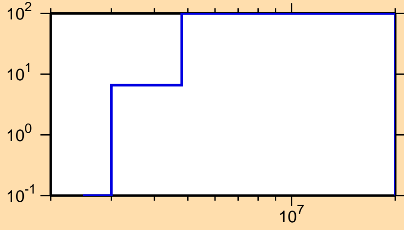
\Delta\sigma/\sigma vs. E for ^{195}\text{Ir}(n,p)
