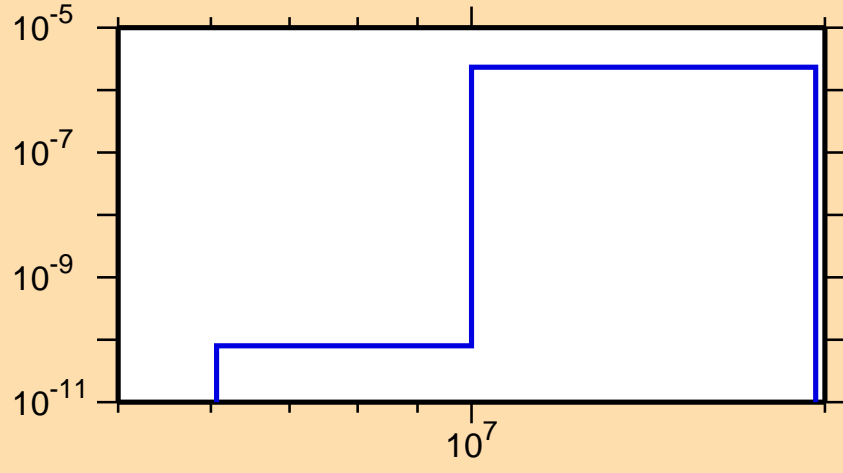
\sigma vs. E for ^{196}\text{Ir}(n,\alpha)
