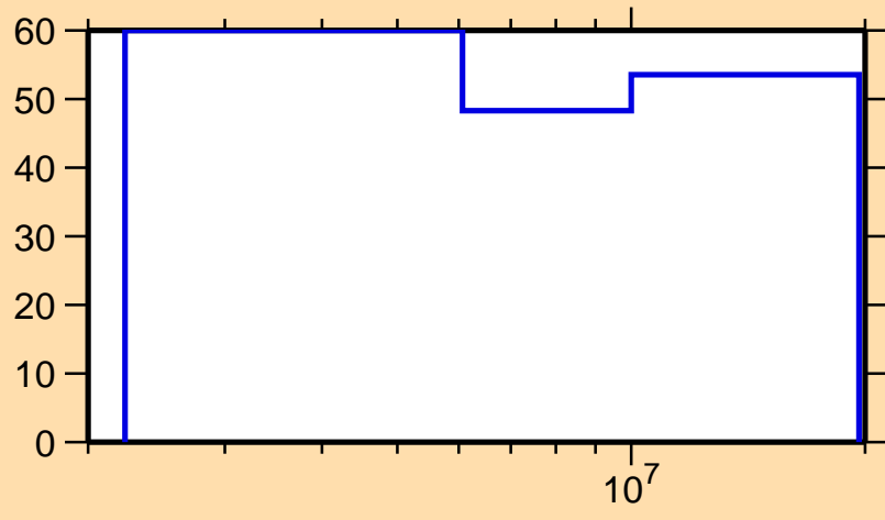
\Delta\sigma/\sigma vs. E for ^{196}\text{Ir}(n,p)
