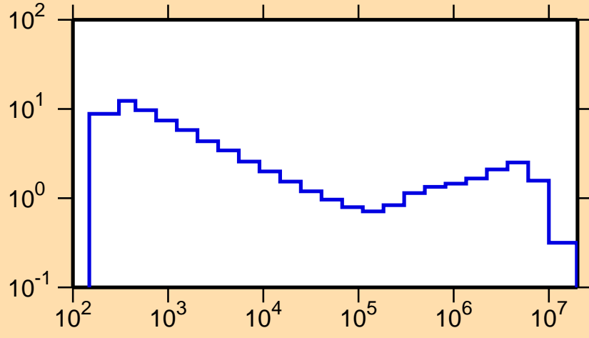
\sigma vs. E for ^{196}\text{Ir}(n,\text{inel.})
