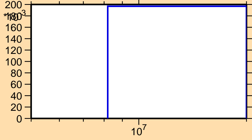
\sigma vs. E for ^{197}\text{Ir}(n,3n)
