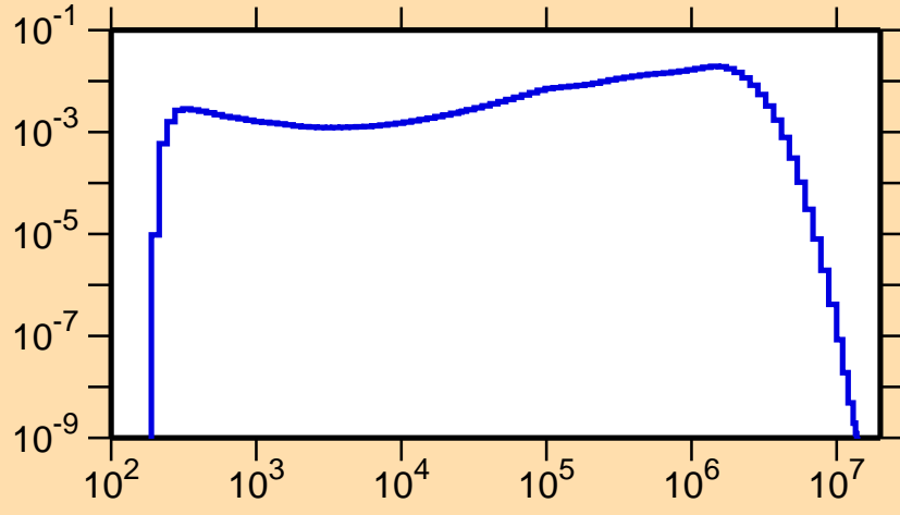
\sigma vs. E for ^{197}\text{Ir}(n,n_1)
