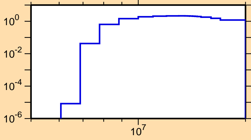
\sigma vs. E for ^{197}\text{Ir}(n,2n)
