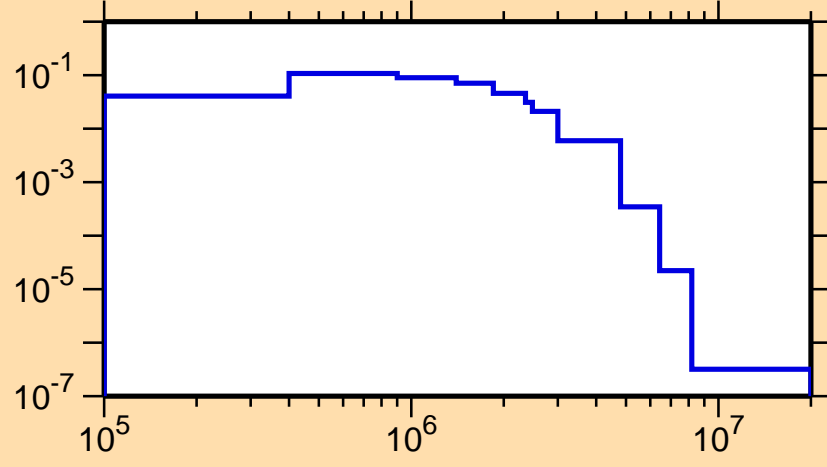
\sigma vs. E for ^{197}\text{Ir}(n,n_4)
