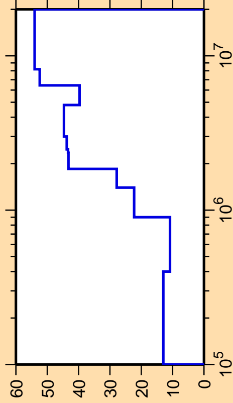
\Delta\sigma/\sigma vs. E for ^{197}\text{Ir}(n,n_4)
