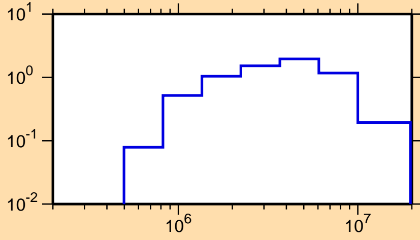
\sigma vs. E for ^{198}\text{Ir}(n,n\text{cont.})
