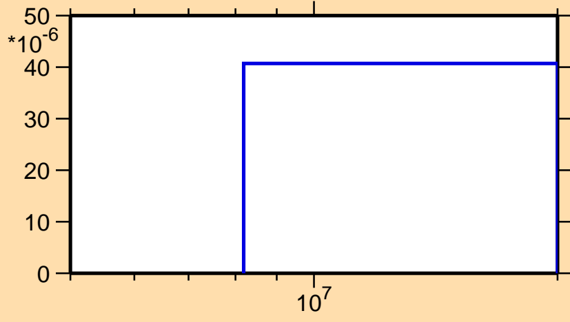
\sigma vs. E for ^{198}\text{Ir}(n,d)
