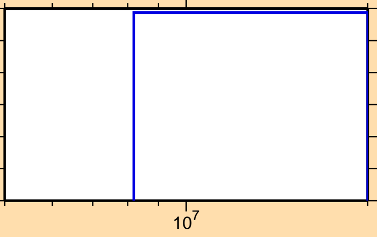
\sigma vs. E for ^{198}\text{Ir}(n,np)
