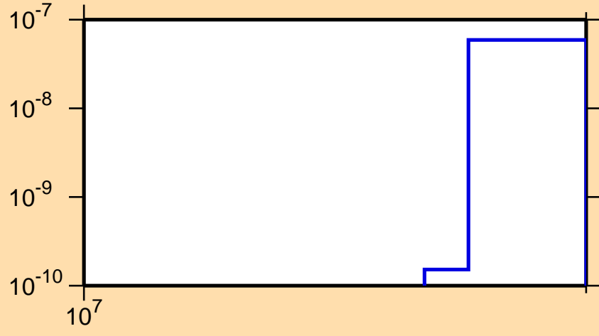
\sigma vs. E for ^{199}\text{Ir}(n,\text{nd})
