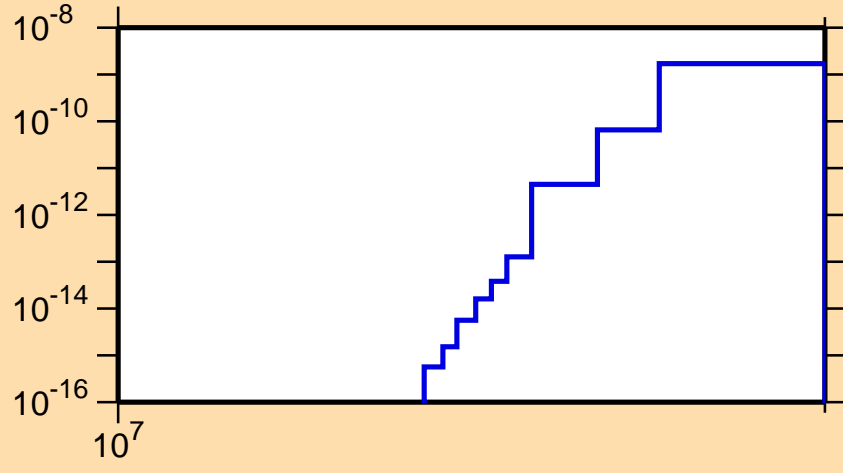
\sigma vs. E for ^{199}\text{Ir}(n,2n\alpha)
