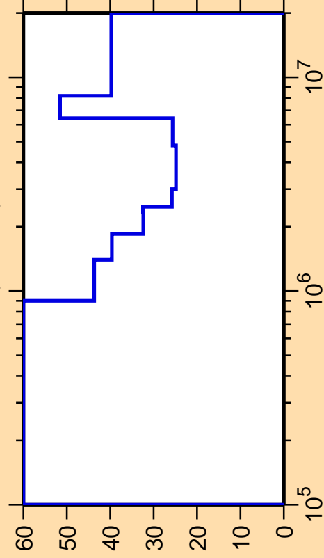
\Delta\sigma/\sigma vs. E for ^{199}\text{Ir}(n,\text{inel.})
