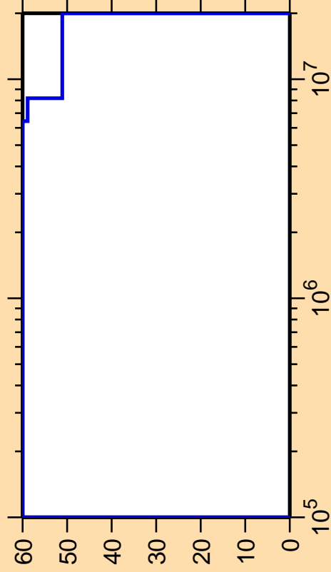
\Delta\sigma/\sigma vs. E for ^{199}\text{Ir}(n,n_2)
