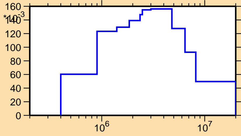
\sigma vs. E for ^{199}\text{Ir}(n,n_4)
