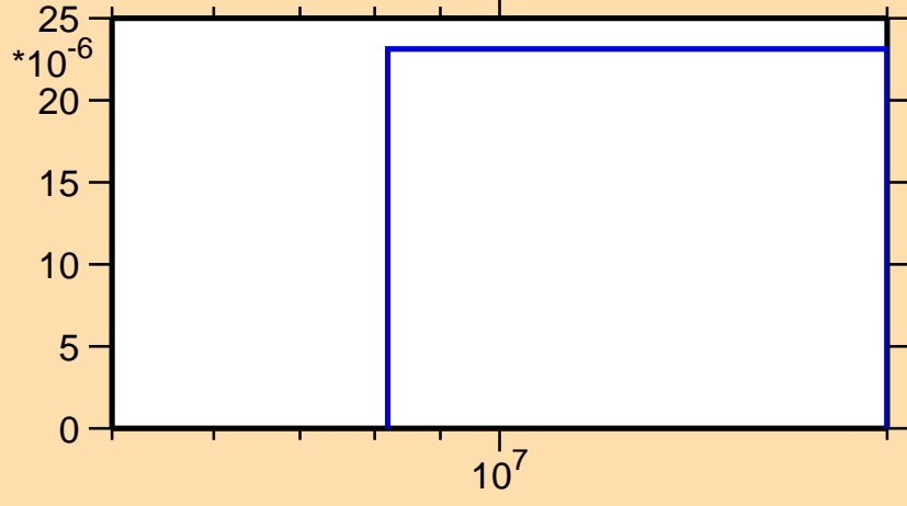
\sigma vs. E for ^{199}\text{Ir}(n,d)
