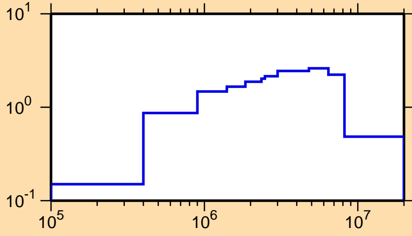
\sigma vs. E for ^{199}\text{Ir}(n,\text{inel.})
