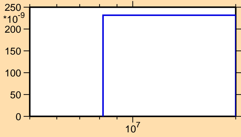
\sigma vs. E for ^{199}\text{Ir}(n,n\alpha)
