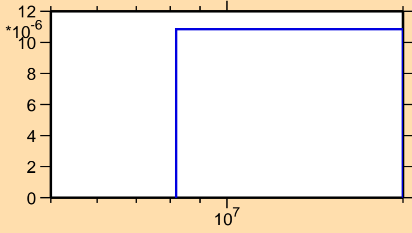
\sigma vs. E for ^{199}\text{Ir}(n,np)
