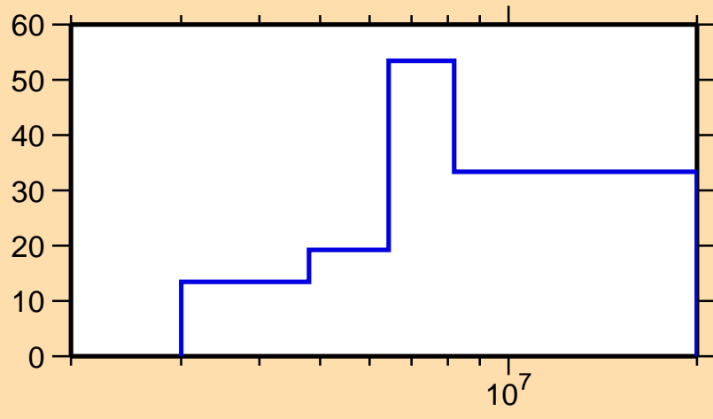
\Delta\sigma/\sigma vs. E for ^{200}\text{Ir}(n,ncont.)
