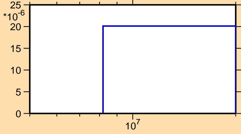
\sigma vs. E for ^{200}\text{Ir}(n,d)
