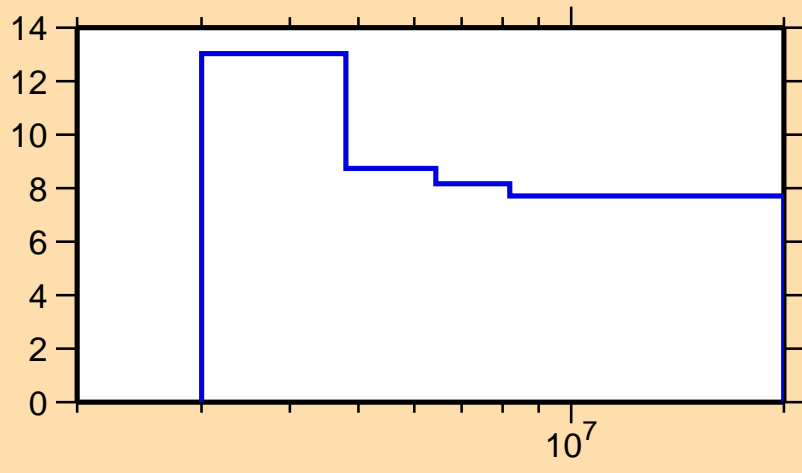
\Delta\sigma/\sigma vs. E for ^{200}\text{Ir}(n,\text{nonel.})
