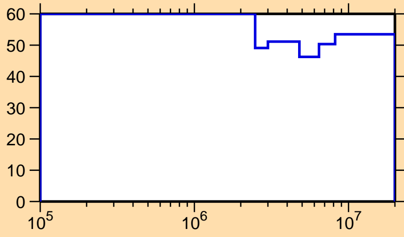
\Delta\sigma/\sigma vs. E for ^{200}\text{Ir}(n,n_1)
