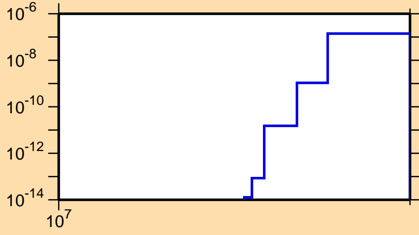
\sigma vs. E for ^{201}\text{Ir}(n,nt)
