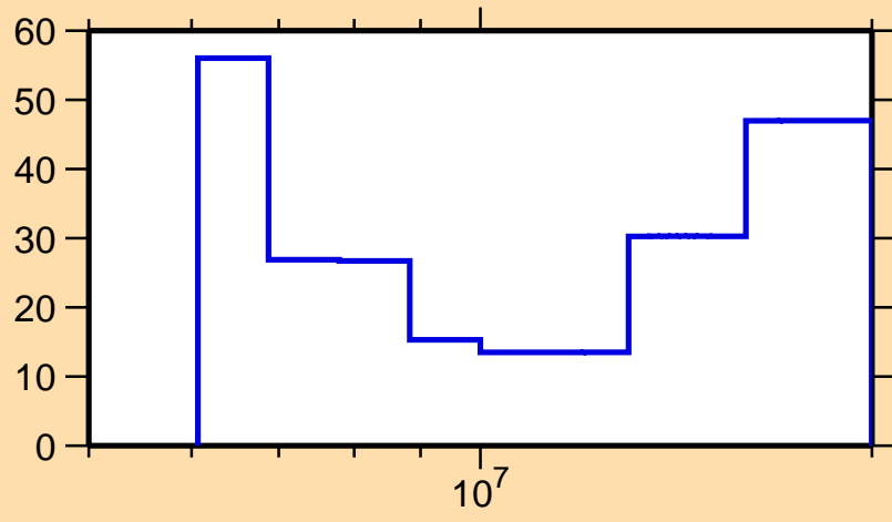
\Delta\sigma/\sigma vs. E for ^{201}\text{Ir}(n,2n)
