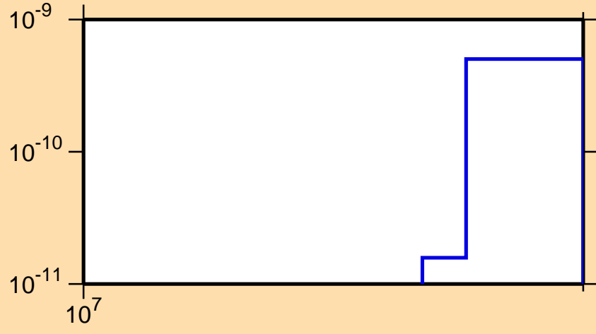
\sigma vs. E for ^{201}\text{Ir}(n,2n\alpha)
