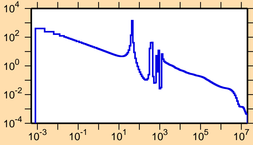
\sigma vs. E for ^{201}\text{Ir}(n,\gamma)
