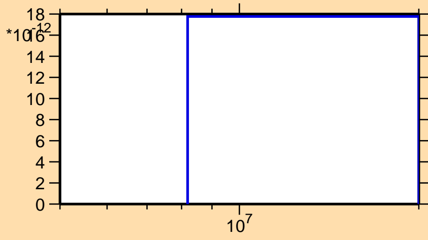
\sigma vs. E for ^{201}\text{Ir}(n,2np)
