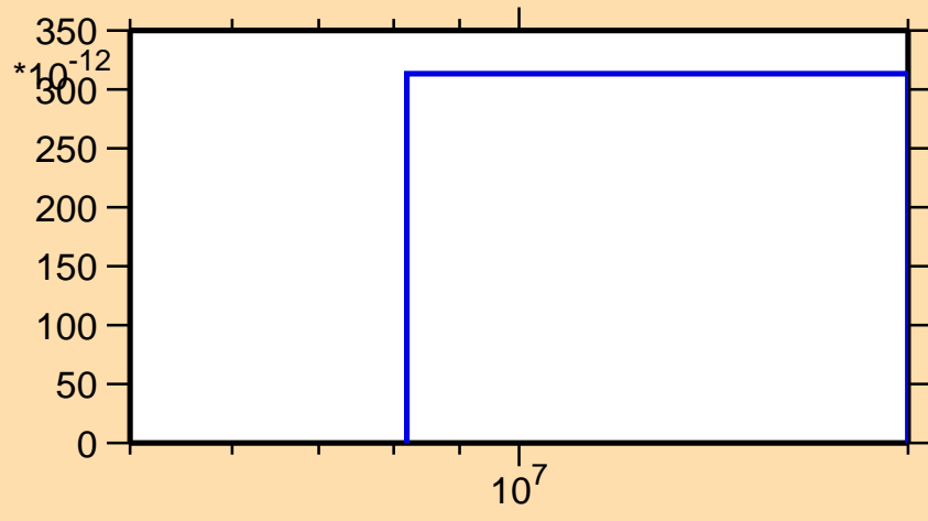
\sigma vs. E for ^{201}\text{Ir}(n,\text{nd})
