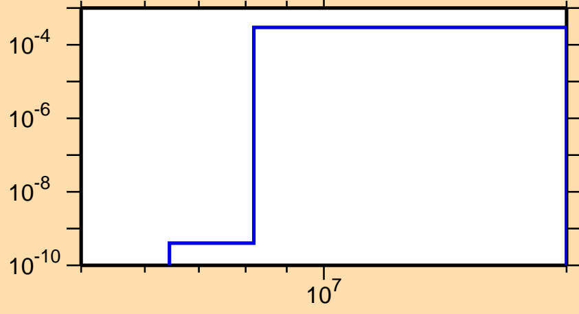
\sigma vs. E for ^{201}\text{Ir}(n,p)
