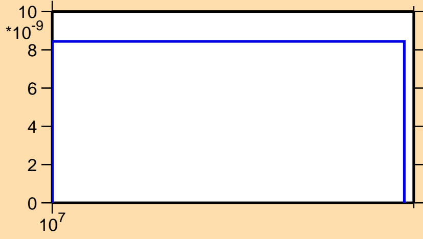
\sigma vs. E for ^{202}\text{Ir}(n,\text{nd})
