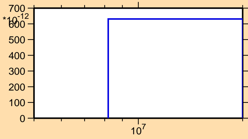
\sigma vs. E for ^{202}\text{Ir}(n,2np)
