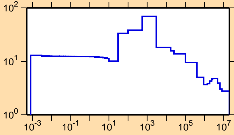
\sigma vs. E for ^{202}\text{Ir}(n,\text{el.})
