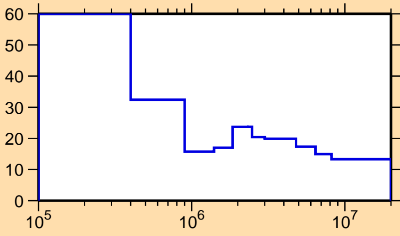
\Delta\sigma/\sigma vs. E for ^{202}\text{Ir}(n,\text{nonel.})
