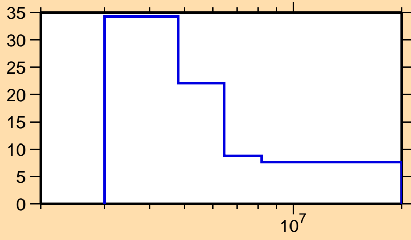
\Delta\sigma/\sigma vs. E for ^{202}\text{Ir}(n,\text{tot.})
