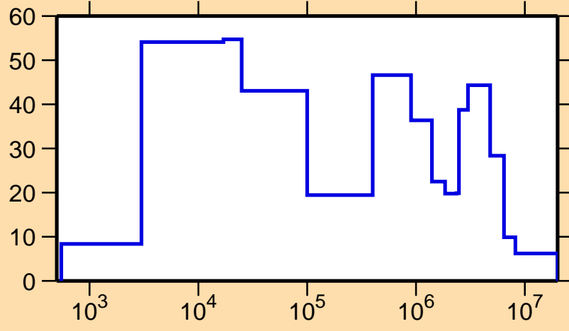
\Delta\sigma/\sigma vs. E for ^{202}\text{Ir}(n,\text{el.})
