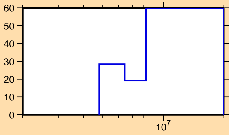
\Delta\sigma/\sigma vs. E for ^{202}\text{Ir}(n,2n)
