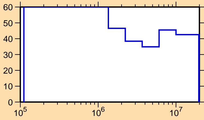
\Delta\sigma/\sigma vs. E for ^{203}\text{Ir}(n,n_1)
