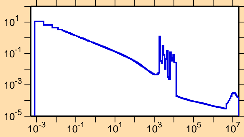
\sigma vs. E for ^{37}\text{K}(n,\gamma)
