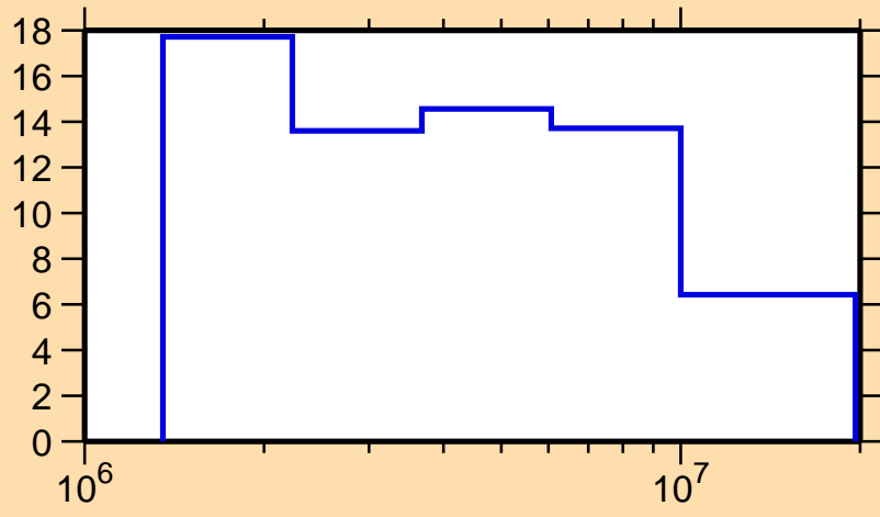
\Delta\sigma/\sigma vs. E for ^{37}\text{K}(n,\text{el.})
