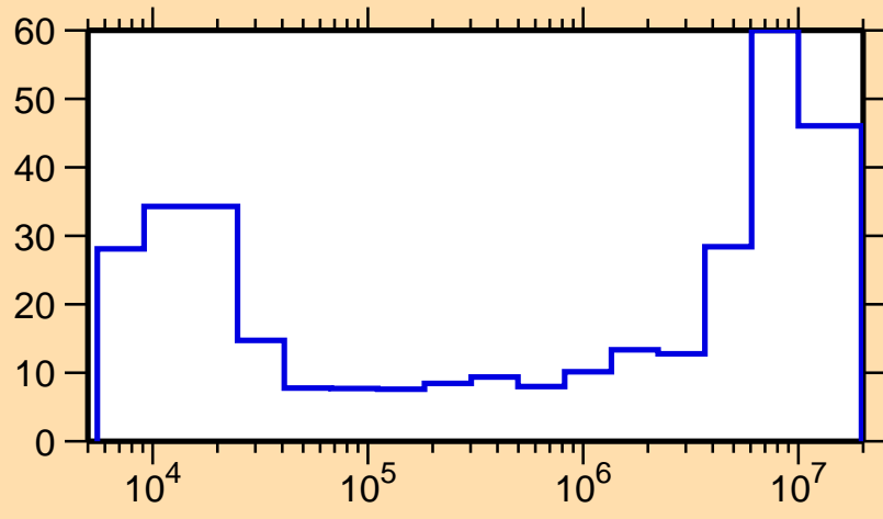
\Delta\sigma/\sigma vs. E for ^{37}\text{K}(n,p)
