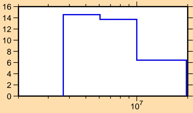
\Delta\sigma/\sigma vs. E for ^{37}\text{K}(n,el.)
