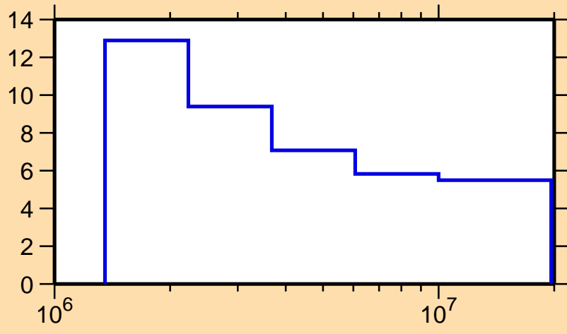
\Delta\sigma/\sigma vs. E for ^{37}\text{K}(n,\text{nonel.})
