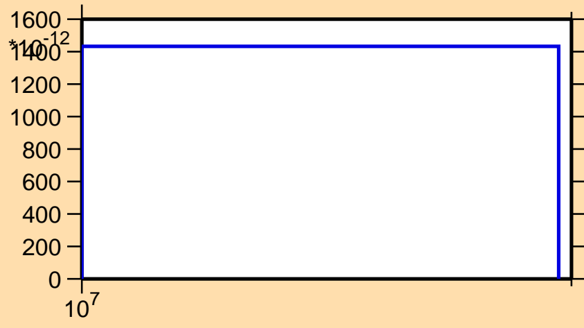
\sigma vs. E for ^{37}\text{K}(n,2np)
