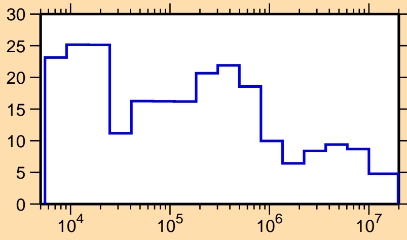
\Delta\sigma/\sigma vs. E for ^{37}\text{K}(n,\text{tot.})
