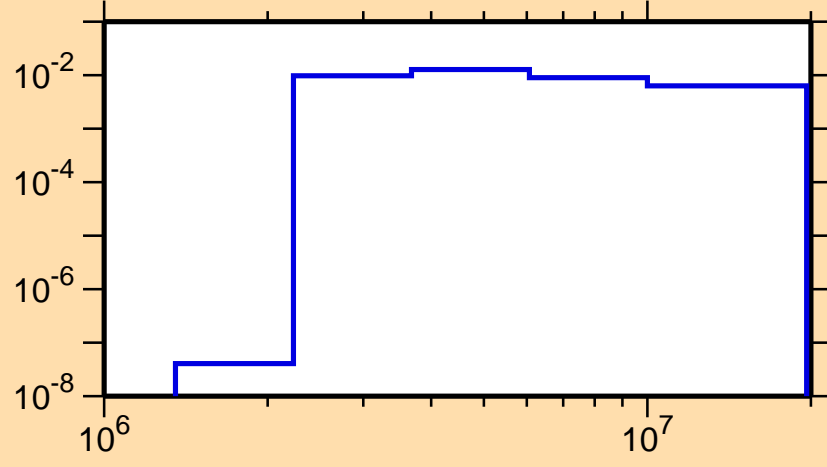
\sigma vs. E for ^{37}\text{K}(n,n_3)
