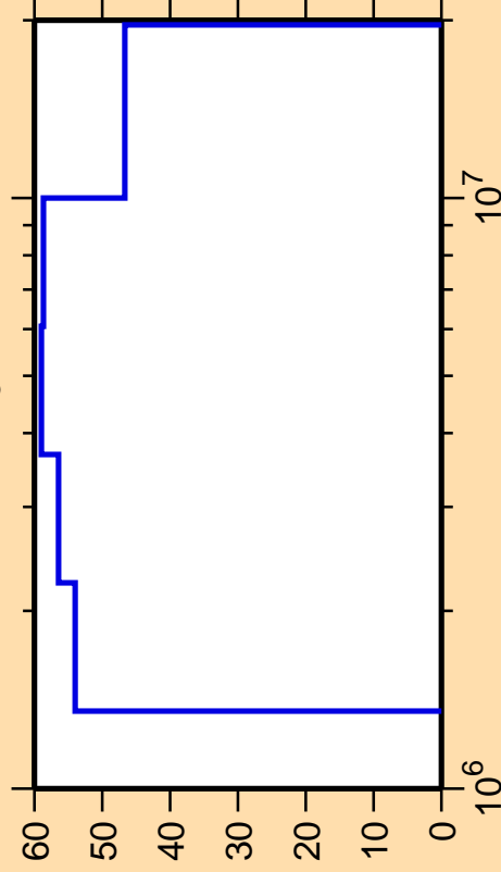
\Delta\sigma/\sigma vs. E for ^{37}\text{K}(n,n_3)
