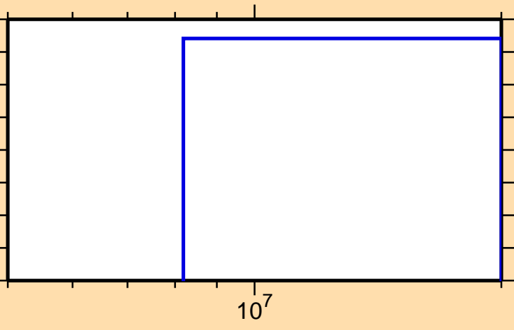
\sigma vs. E for ^{37}\text{K}(n,n\alpha)
