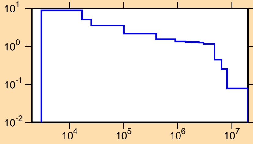
\sigma vs. E for ^{37}\text{K}(n,p)
