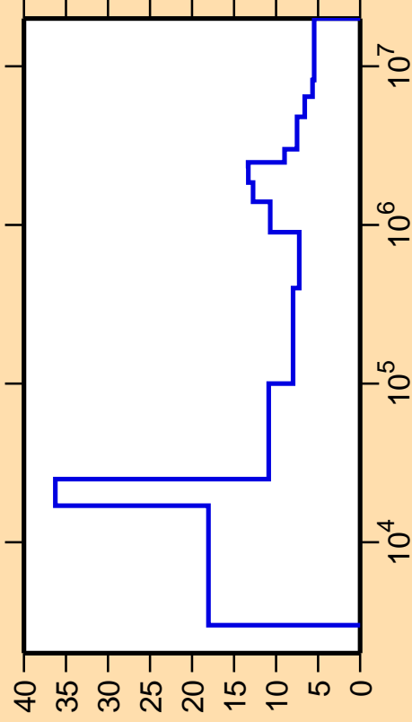
\Delta\sigma/\sigma vs. E for ^{37}\text{K}(n,\text{nonel.})
