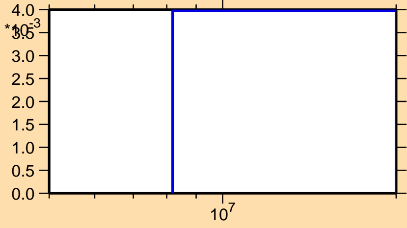
\sigma vs. E for ^{37}\text{K}(n,\text{pd})
