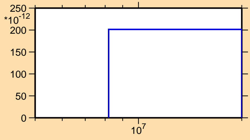
\sigma vs. E for ^{37}\text{K}(\text{mt } 34)
