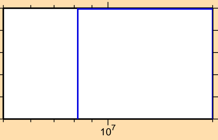
\sigma vs. E for ^{37}\text{K}(n,nd)
