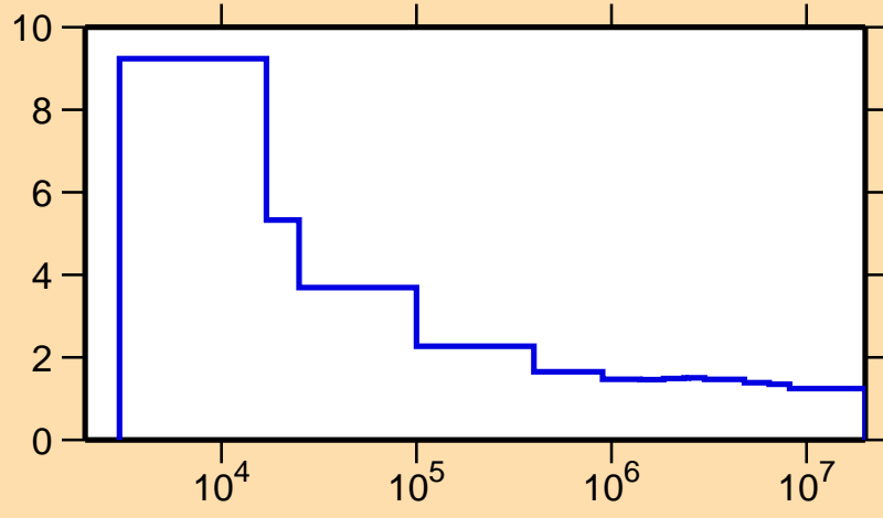
\sigma vs. E for ^{37}\text{K}(n,\text{nonel.})
