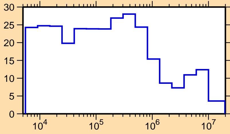
\Delta\sigma/\sigma vs. E for ^{38}\text{K}(n,el.)
