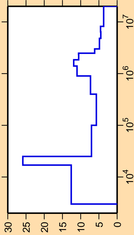
\Delta\sigma/\sigma vs. E for ^{38}\text{K}(n,\text{nonel.})
