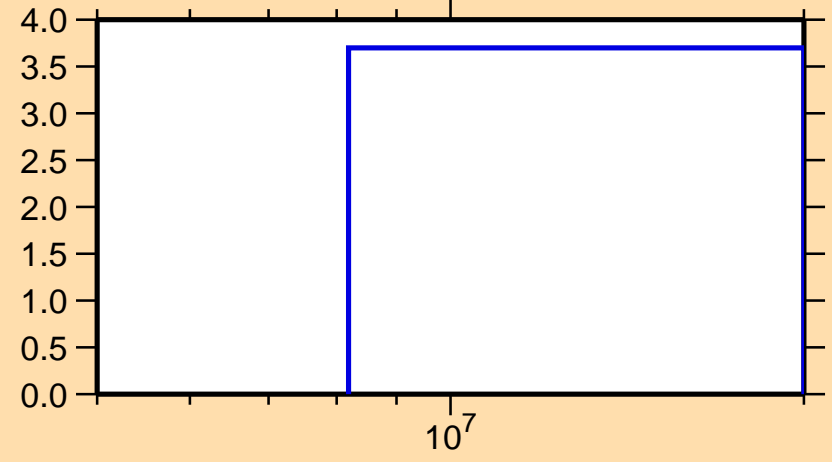
\Delta\sigma/\sigma vs. E for ^{38}\text{K}(n,\text{nonel.})
