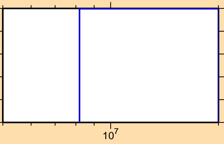
\sigma vs. E for ^{38}\text{K}(n,\text{pt})
