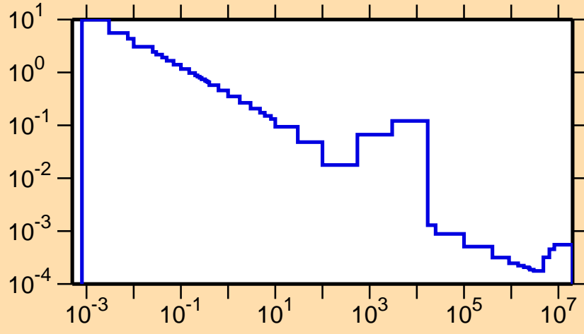
\sigma vs. E for ^{38}\text{K}(n,\gamma)
