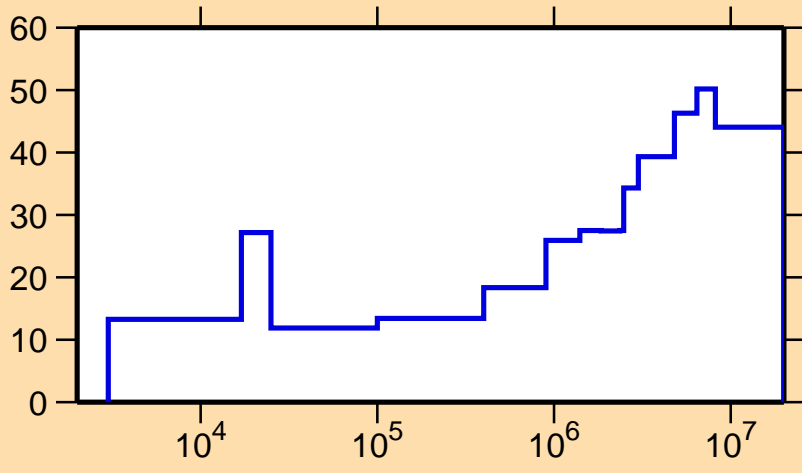
\Delta\sigma/\sigma vs. E for ^{38}\text{K}(n,p)
