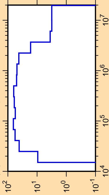
\Delta\mu/\mu vs. E for ^{39}\text{K}(\text{mt251})
