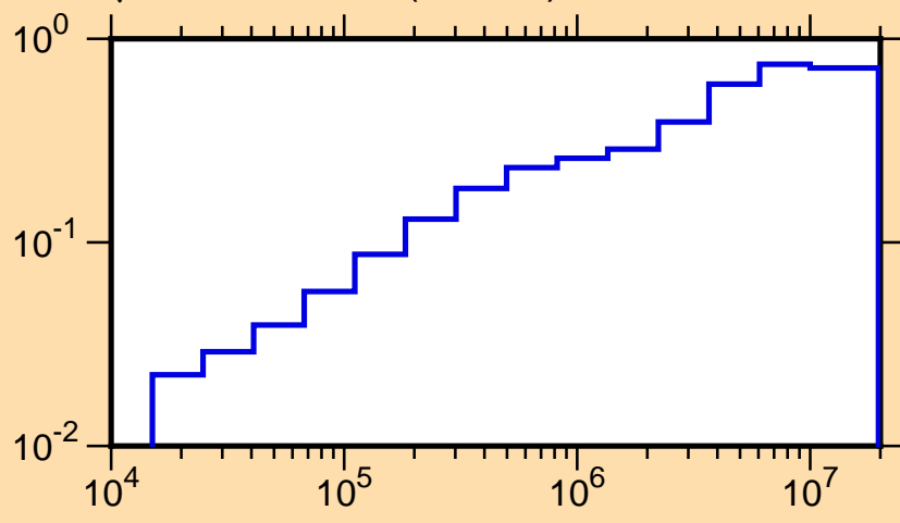
\mu vs. E for ^{39}\text{K}(\text{mt251})
