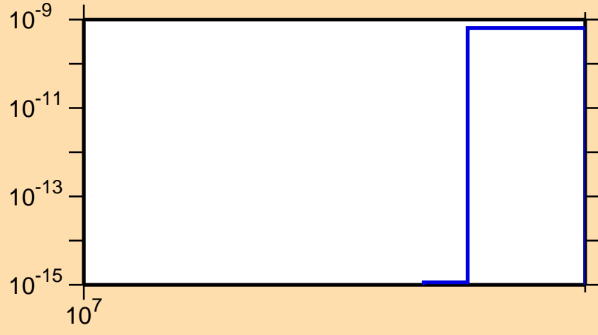
\sigma vs. E for ^{40}\text{K}(n,\text{pd})
