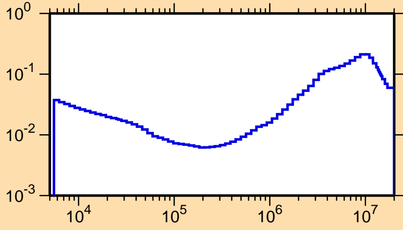
\sigma vs. E for ^{40}\text{K}(n,p)
