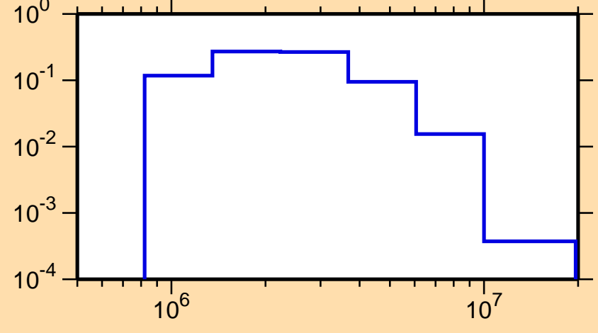
\sigma vs. E for ^{40}\text{K}(n,n_3)
