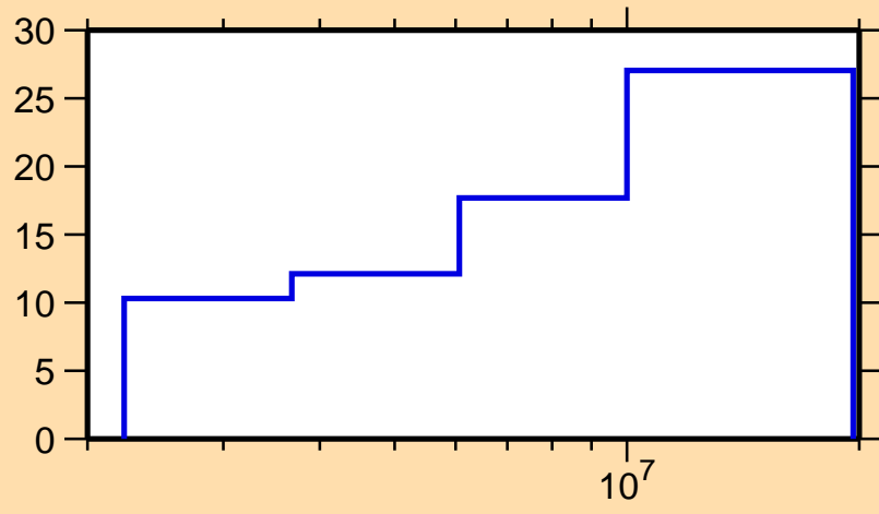
\Delta\sigma/\sigma vs. E for ^{40}\text{K}(n,inel.)
