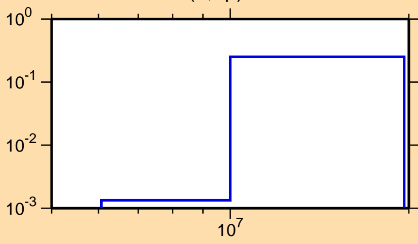
\sigma vs. E for ^{40}\text{K}(n,np)
