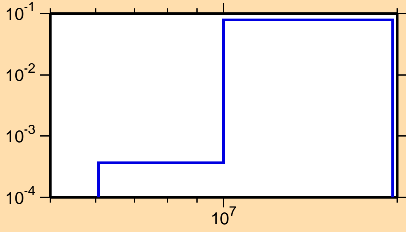
\sigma vs. E for ^{41}\text{K}(n,n\alpha)
