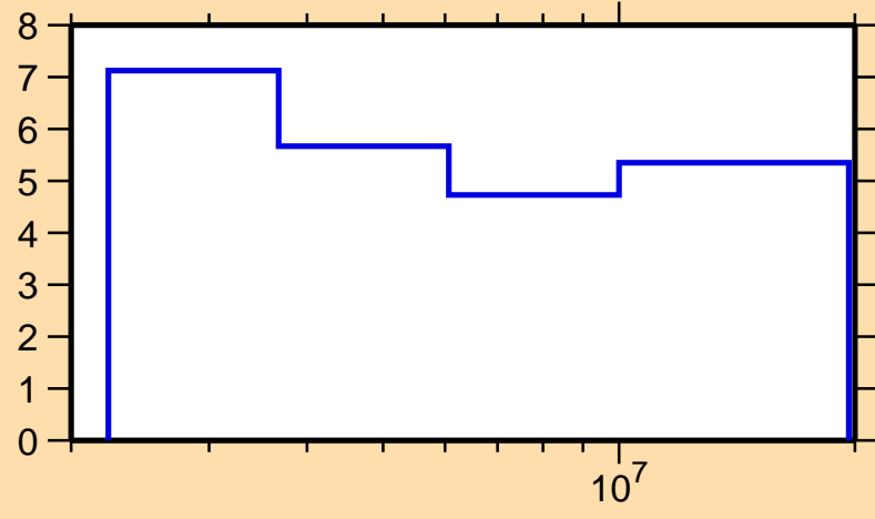
\Delta\sigma/\sigma vs. E for ^{41}\text{K}(n,n\text{onel.})
