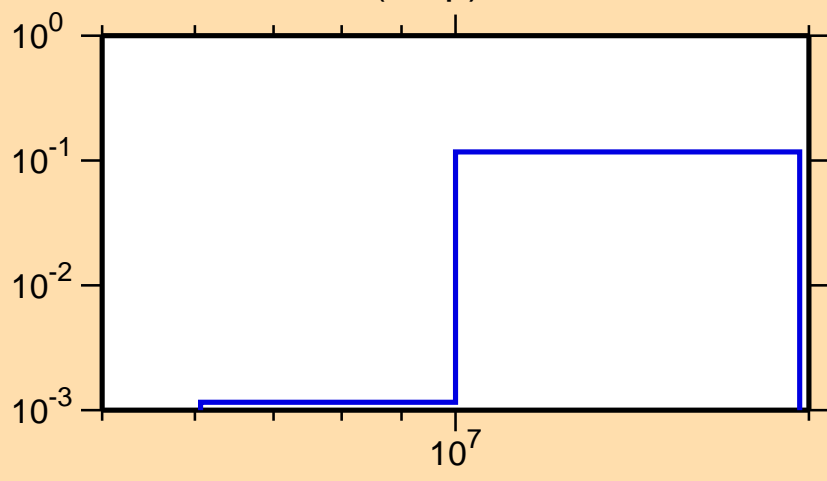
\sigma vs. E for ^{41}\text{K}(n,np)
