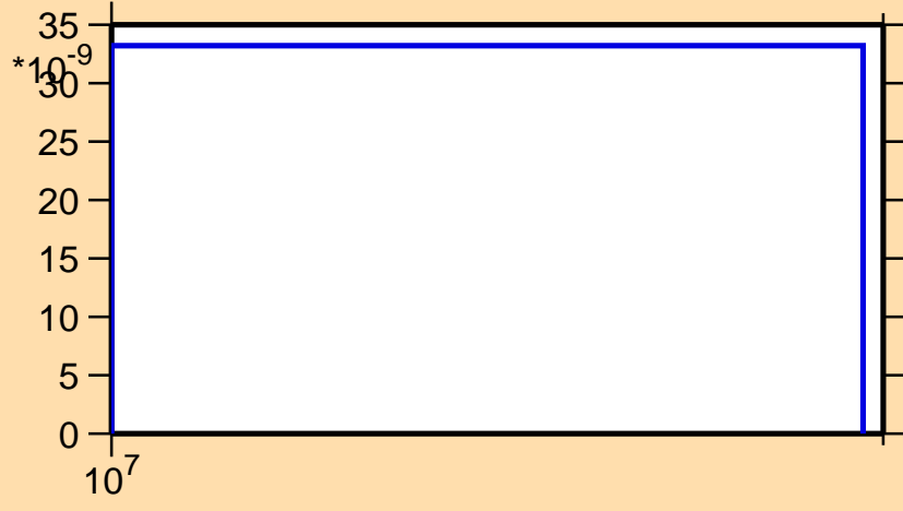
\sigma vs. E for ^{41}\text{K}(n,nt)
