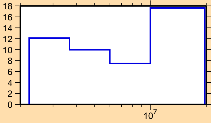
\Delta\sigma/\sigma vs. E for ^{41}\text{K}(n,ncont.)
