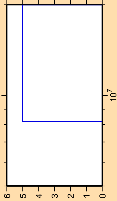
\Delta\sigma/\sigma vs. E for ^{41}\text{K}(n,2n\alpha)
