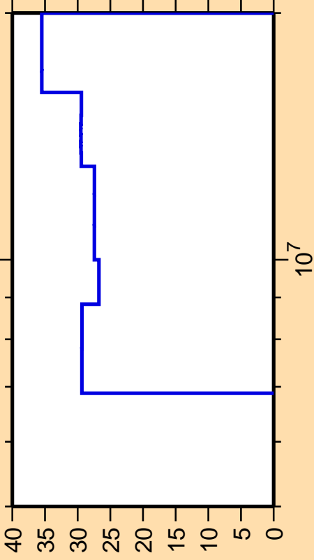
\Delta\sigma/\sigma vs. E for ^{42}\text{K}(n,p)
