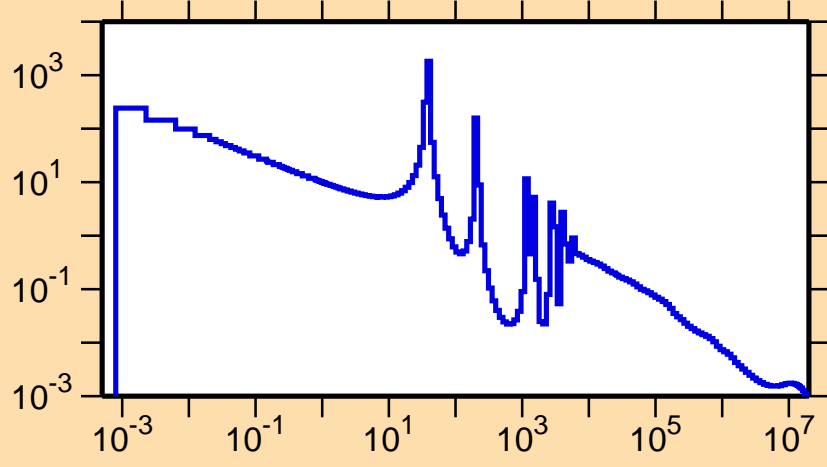
\sigma vs. E for ^{42}\text{K}(n,\gamma)
