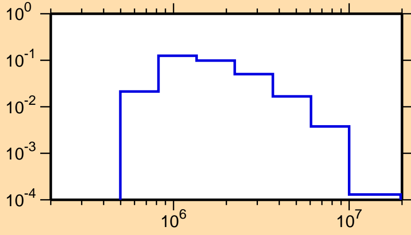
\sigma vs. E for ^{42}\text{K}(n,n_4)
