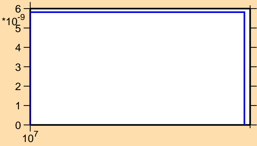
\sigma vs. E for ^{42}\text{K}(n,nt)
