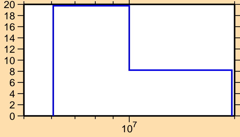
\Delta\sigma/\sigma vs. E for ^{42}\text{K}(n,\text{el.})
