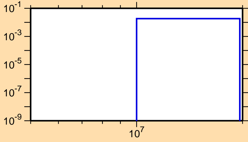
\sigma vs. E for ^{42}\text{K}(n,n\alpha)
