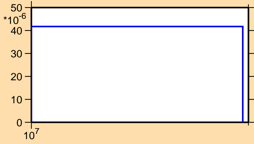
\sigma vs. E for ^{42}\text{K}(n,nd)
