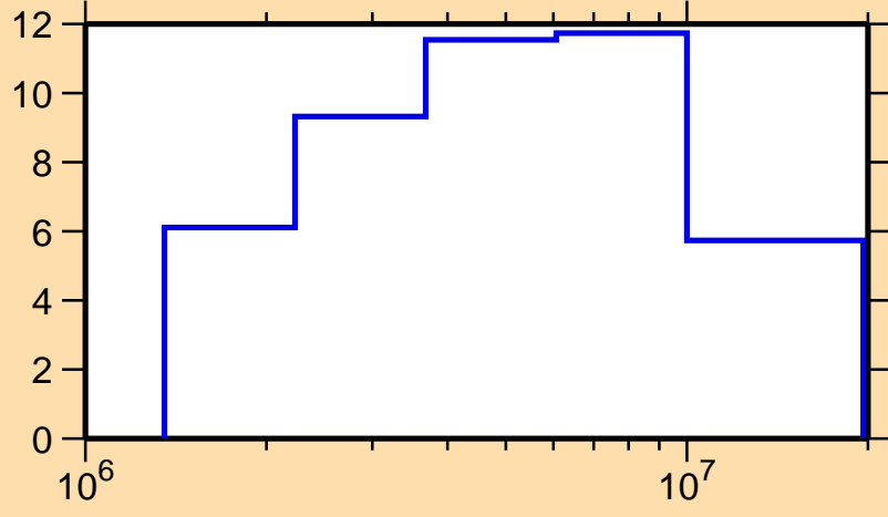
\Delta\sigma/\sigma vs. E for ^{42}\text{K}(n,tot.)
