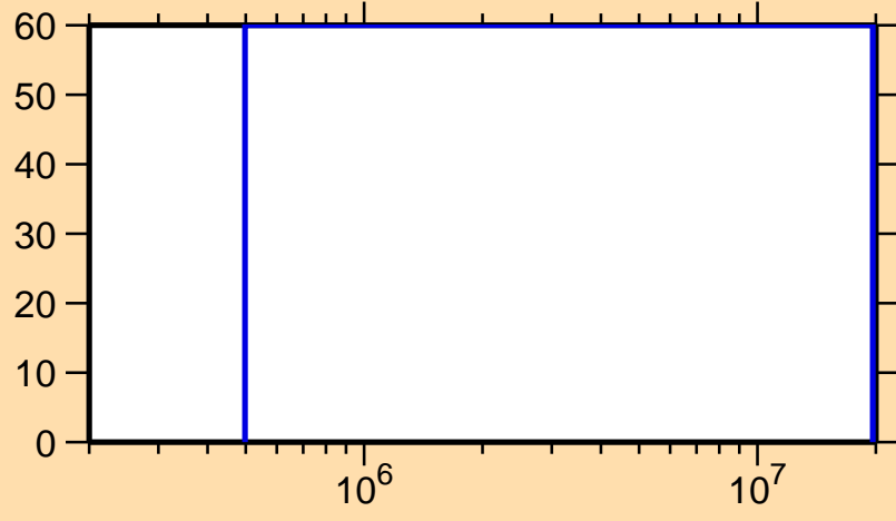
\Delta\sigma/\sigma vs. E for ^{42}\text{K}(n,\gamma)
