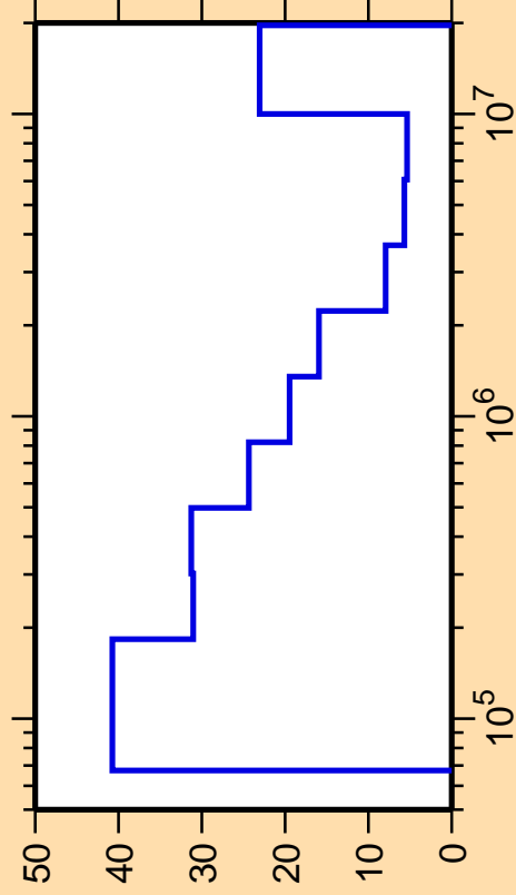
\Delta\sigma/\sigma vs. E for ^{42}\text{K}(n,\text{inel.})
