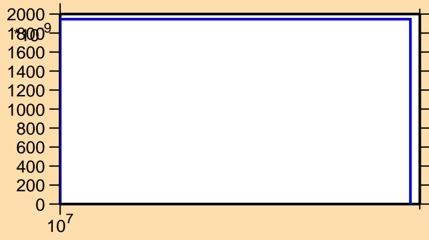
\sigma vs. E for ^{42}\text{K}(n,2n\alpha)
