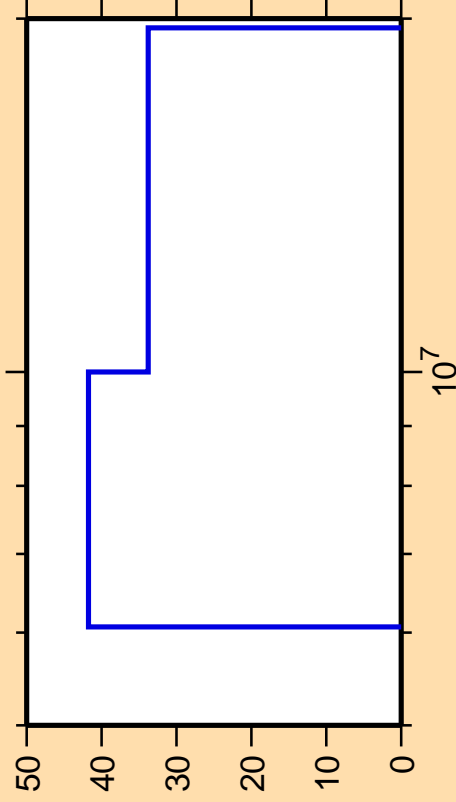
\Delta\sigma/\sigma vs. E for ^{42}\text{K}(n,n_1)
