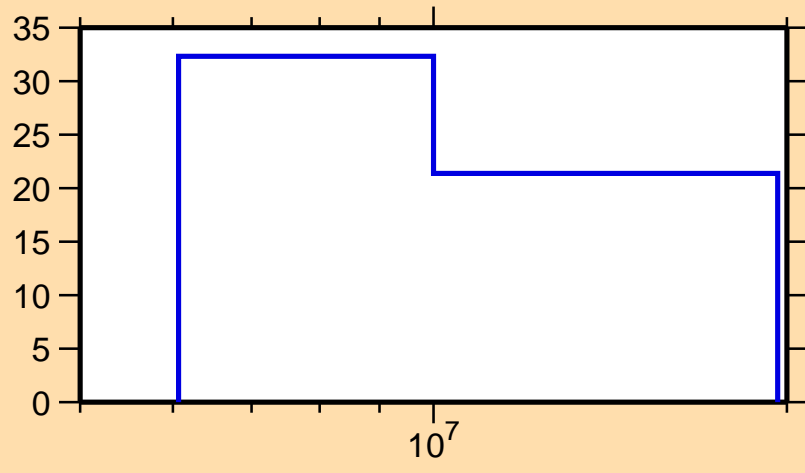
\Delta\sigma/\sigma vs. E for ^{42}\text{K}(n,2n)
