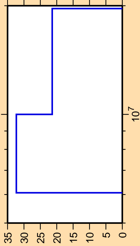
\Delta\sigma/\sigma vs. E for ^{42}\text{K}(n,2n)
