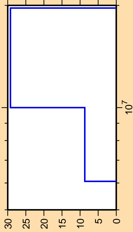
\Delta\sigma/\sigma vs. E for ^{42}\text{K}(n,n\text{cont.})
