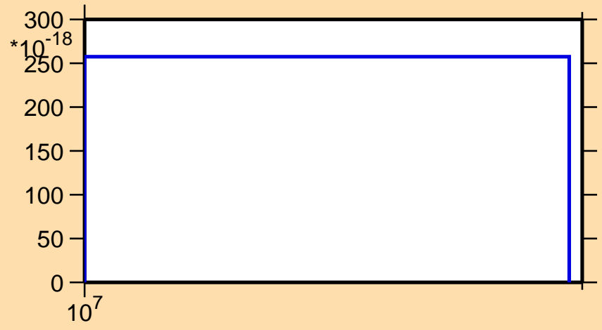
\sigma vs. E for ^{42}\text{K}(\text{mt117})
