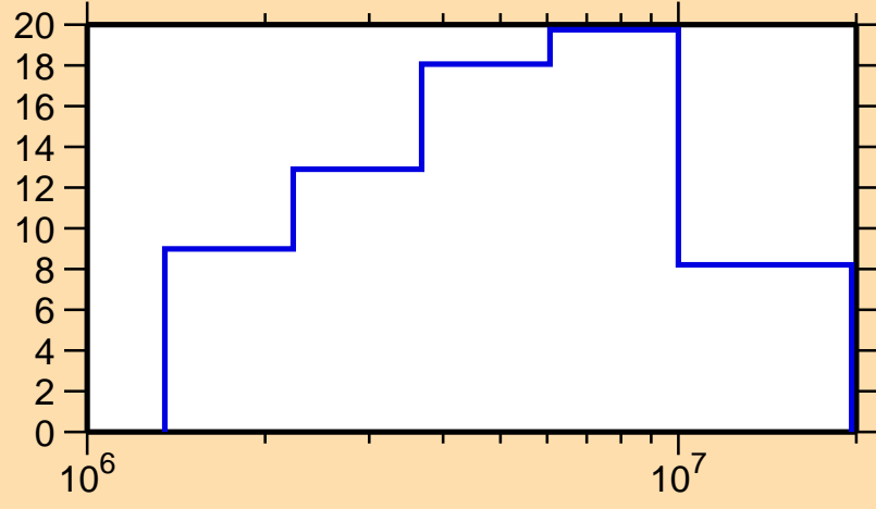
\Delta\sigma/\sigma vs. E for ^{42}\text{K}(n,el.)
