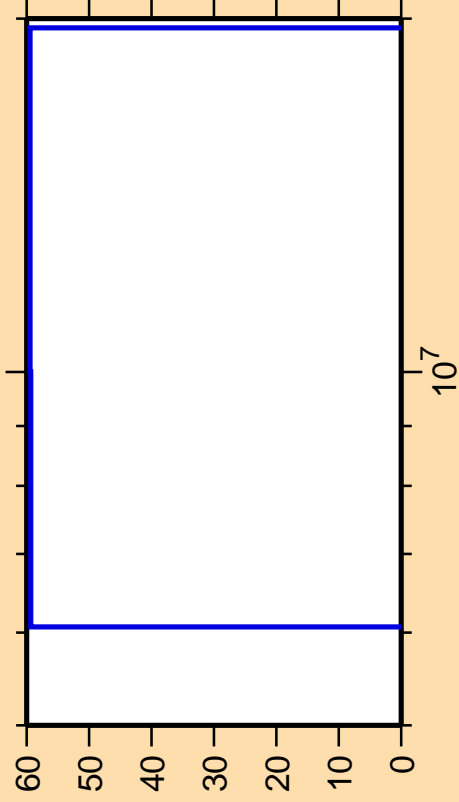
\Delta\sigma/\sigma vs. E for ^{42}\text{K}(n,np)
