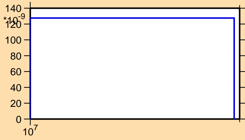
\sigma vs. E for ^{42}\text{K}(n,p\alpha)
