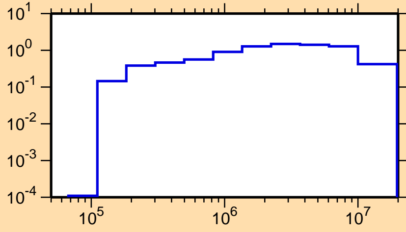
\sigma vs. E for ^{42}\text{K}(n,\text{inel.})
