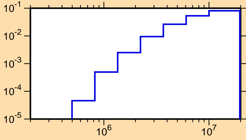
\sigma vs. E for ^{42}\text{K}(n,p)
