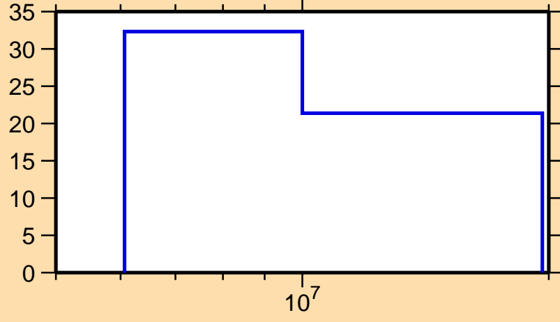
\Delta\sigma/\sigma vs. E for ^{42}\text{K}(n,2n)
