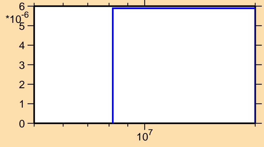
\sigma vs. E for ^{42}\text{K}(n,2np)
