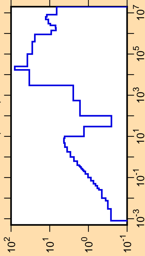
\Delta\sigma/\sigma vs. E for ^{42}\text{K}(n,\text{tot.})
