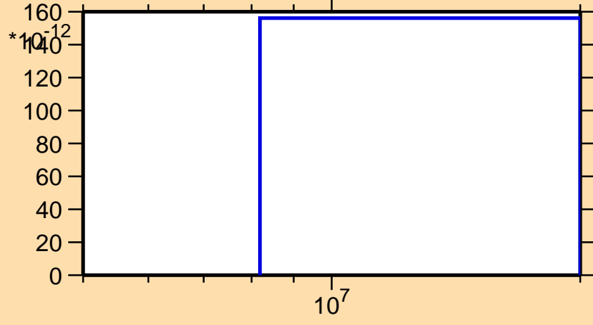
\sigma vs. E for ^{42}\text{K}(n,\text{He}3)
