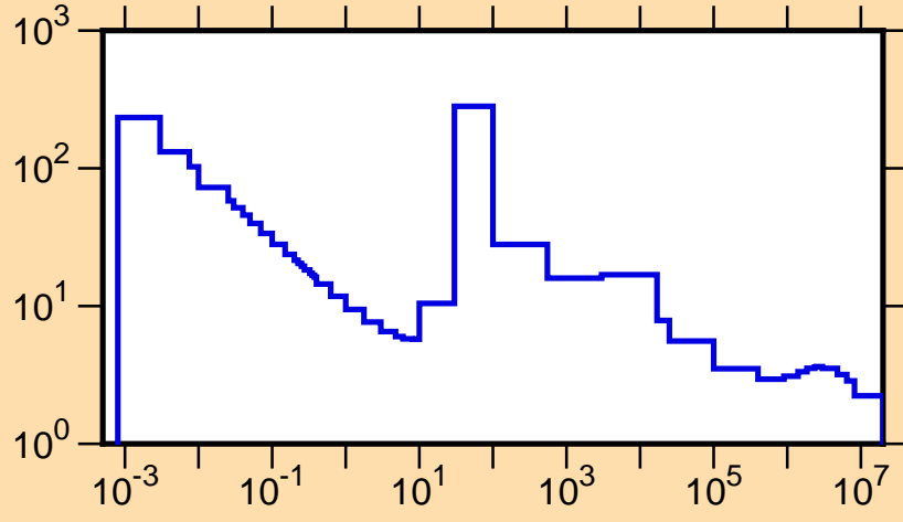
\sigma vs. E for ^{42}\text{K}(n,\text{tot.})
