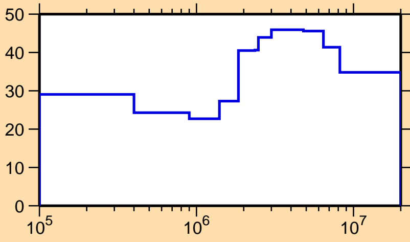
\Delta\sigma/\sigma vs. E for ^{42}\text{K}(n,n_1)
