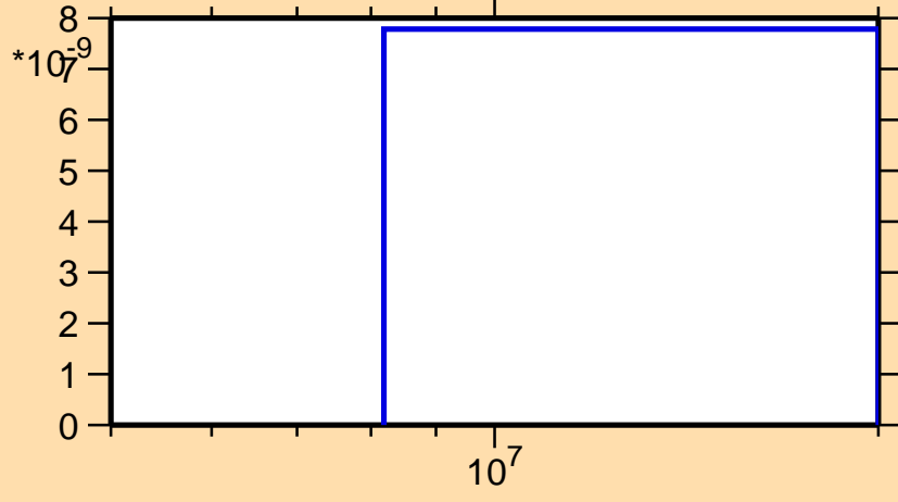
\sigma vs. E for ^{42}\text{K}(n,nt)
