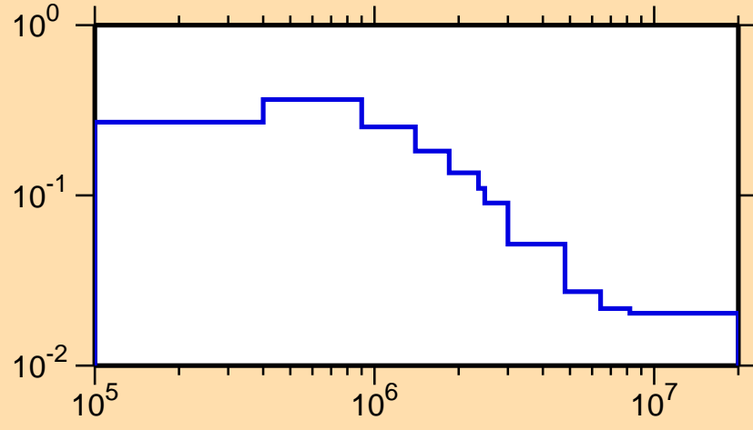
\sigma vs. E for ^{42}\text{K}(n,n_1)
