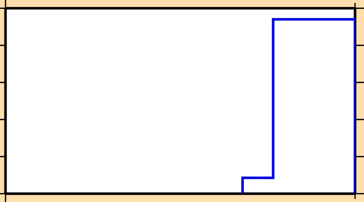
\sigma vs. E for ^{43}\text{K}(n,nt)
