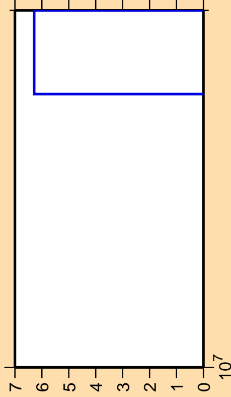
\Delta\sigma/\sigma vs. E for ^{43}\text{K}(n,2n\alpha)
