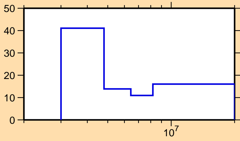
\Delta\sigma/\sigma vs. E for ^{43}\text{K}(n,ncont.)
