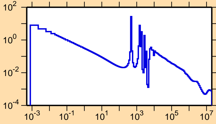
\sigma vs. E for ^{44}\text{K}(n,\gamma)
