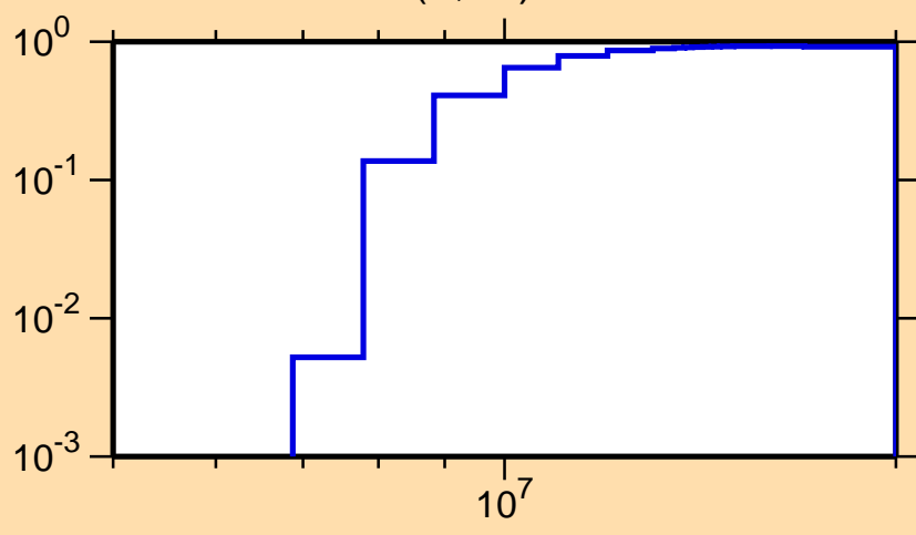
\sigma vs. E for ^{44}\text{K}(n,2n)
