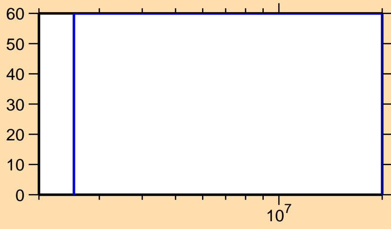
\Delta\sigma/\sigma vs. E for ^{44}\text{K}(n,\gamma)
