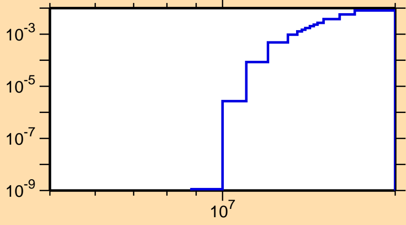
\sigma vs. E for ^{44}\text{K}(n,d)
