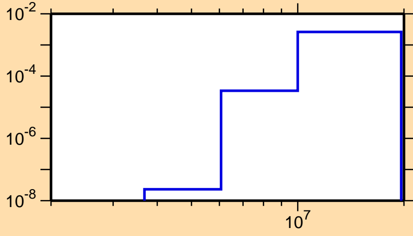
\sigma vs. E for ^{44}\text{K}(n,\alpha)
