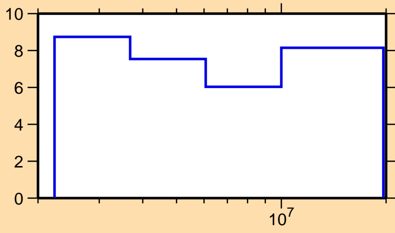
\Delta\sigma/\sigma vs. E for ^{44}\text{K}(n,n\text{onel.})
