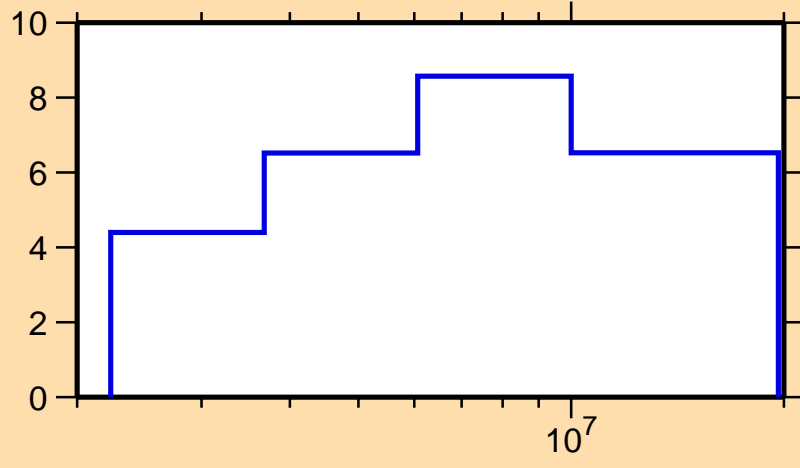
\Delta\sigma/\sigma vs. E for ^{44}\text{K}(n,tot.)
