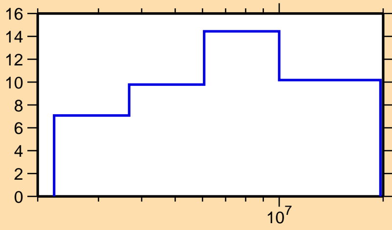
\Delta\sigma/\sigma vs. E for ^{44}\text{K}(n,el.)
