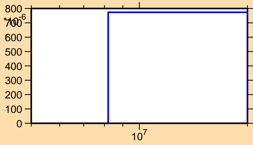
\sigma vs. E for ^{44}\text{K}(n,np)
