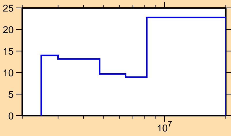
\Delta\sigma/\sigma vs. E for ^{44}\text{K}(n,n\text{cont.})
