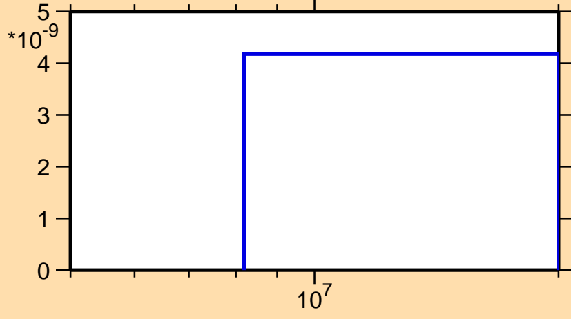
\sigma vs. E for ^{44}\text{K}(n,2np)
