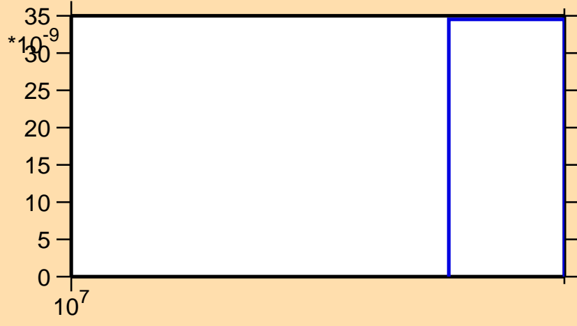
\sigma vs. E for ^{45}\text{K}(n,nt)
