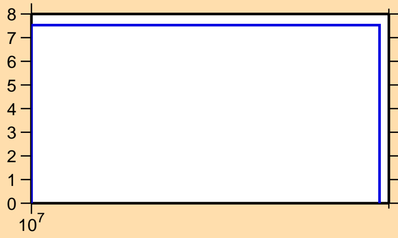
\Delta\sigma/\sigma vs. E for ^{45}\text{K}(n,\text{el.})
