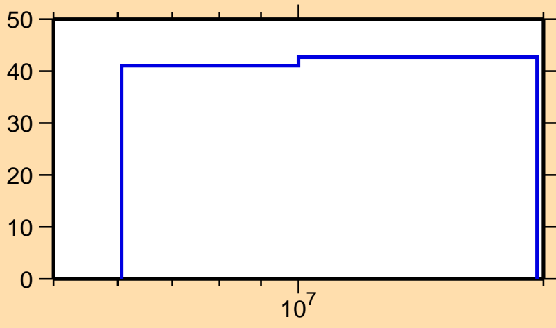
\Delta\sigma/\sigma vs. E for ^{45}\text{K}(n,n\text{cont.})
