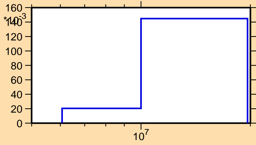
\sigma vs. E for ^{45}\text{K}(n,n\text{cont.})
