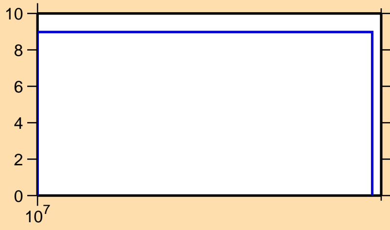
\Delta\sigma/\sigma vs. E for ^{45}\text{K}(n,\text{nonel.})
