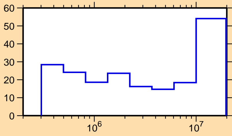
\Delta\sigma/\sigma vs. E for ^{45}\text{K}(n,n_1)
