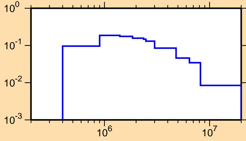
\sigma vs. E for ^{45}\text{K}(n,n_1)
