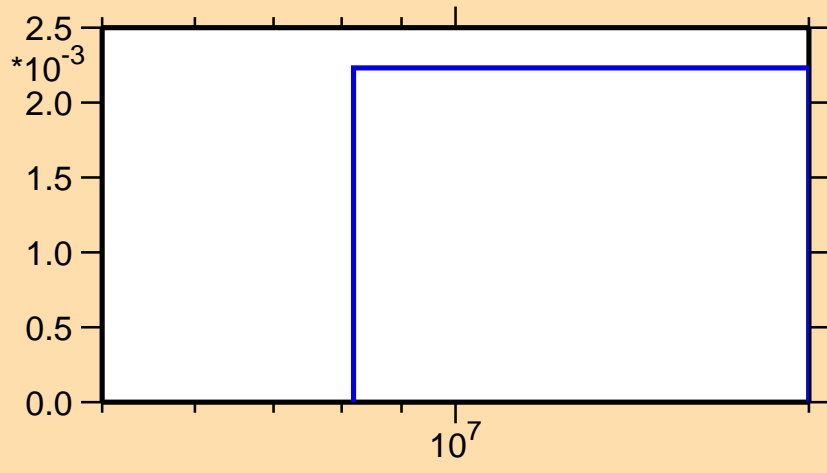
\sigma vs. E for ^{45}\text{K}(n,d)
