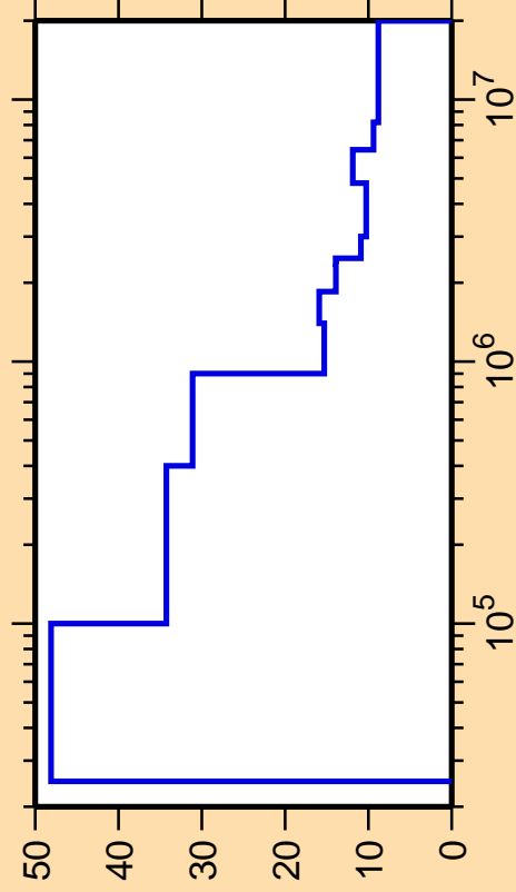
\Delta\sigma/\sigma vs. E for ^{45}\text{K}(n,\text{nonel.})
