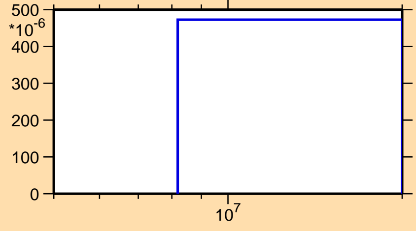
\sigma vs. E for ^{45}\text{K}(n,np)
