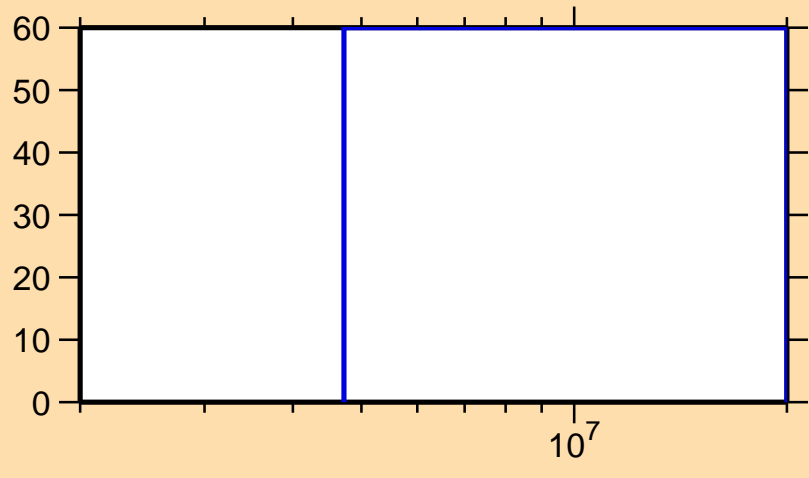
\Delta\sigma/\sigma vs. E for ^{46}\text{K}(n,\gamma)
