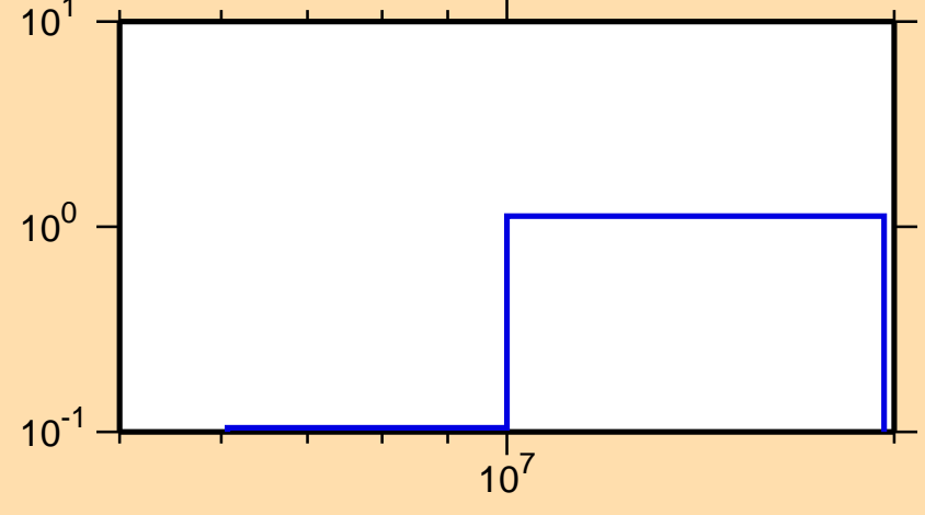
\sigma vs. E for ^{46}\text{K}(n,2n)
