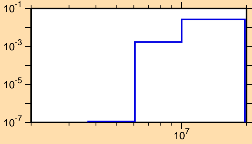
\sigma vs. E for ^{46}\text{K}(n,p)
