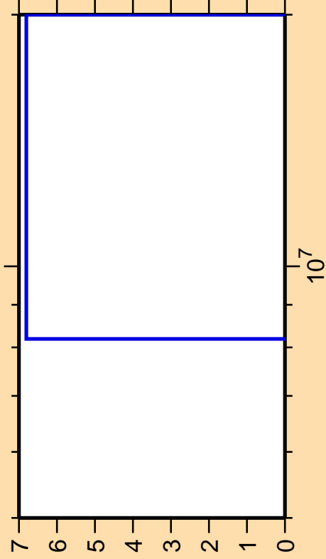
\Delta\sigma/\sigma vs. E for ^{46}\text{K}(n,2n)
