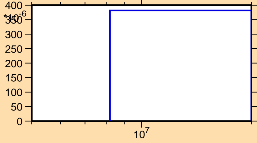
\sigma vs. E for ^{46}\text{K}(n,3n)
