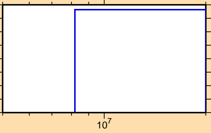
\sigma vs. E for ^{46}\text{K}(n,3n)
