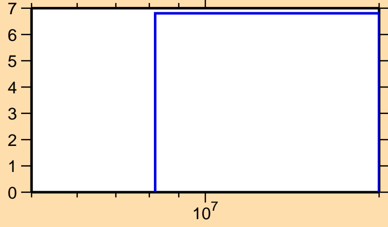
\Delta\sigma/\sigma vs. E for ^{46}\text{K}(n,2n)
