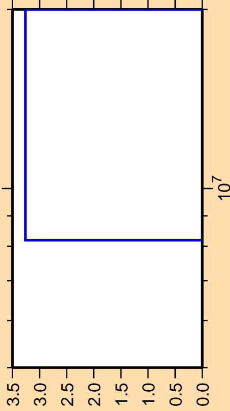
\Delta\sigma/\sigma vs. E for ^{46}\text{K}(n,nt)
