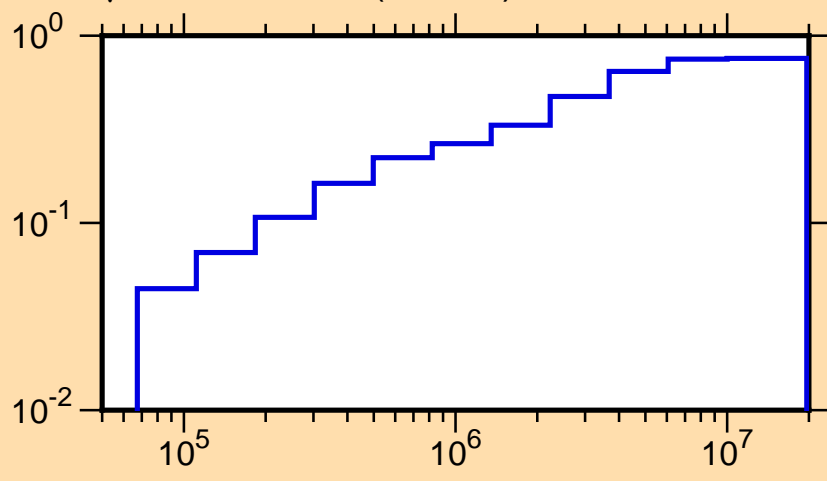
\mu vs. E for ^{47}\text{K}(\text{mt251})
