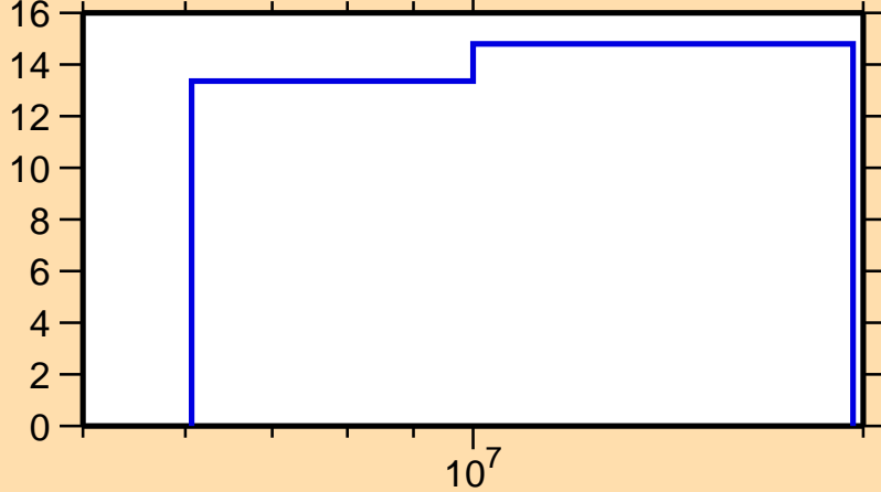
\Delta\sigma/\sigma vs. E for ^{47}\text{K}(n,\text{tot.})
