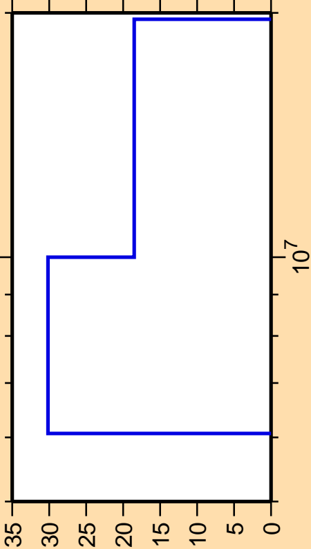
\Delta\sigma/\sigma vs. E for ^{47}\text{K}(n,2n)
