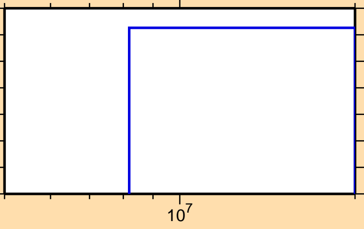
\sigma vs. E for ^{47}\text{K}(n,n\alpha)
