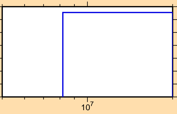
\sigma vs. E for ^{47}\text{K}(n,d)
