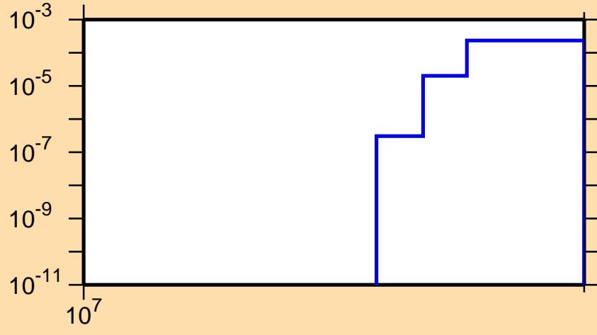
\sigma vs. E for ^{48}\text{K}(n,np)
