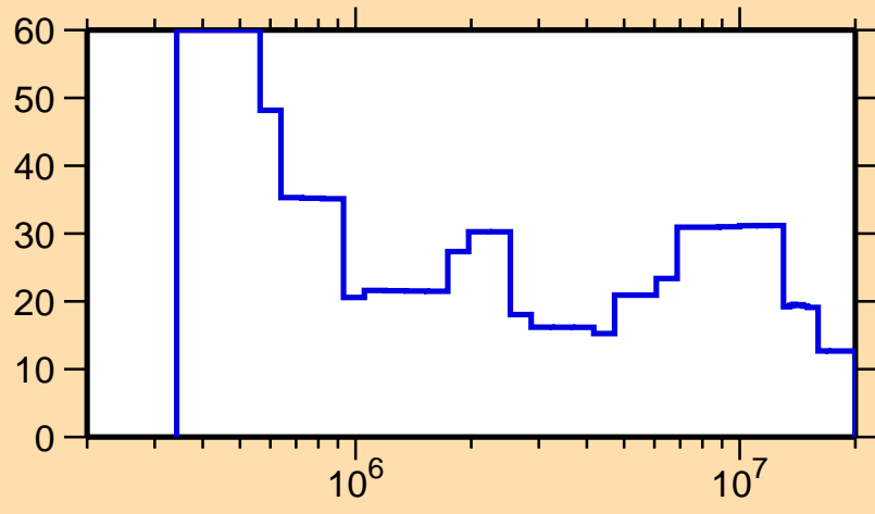
\Delta\sigma/\sigma vs. E for ^{48}\text{K}(n,\text{tot.})
