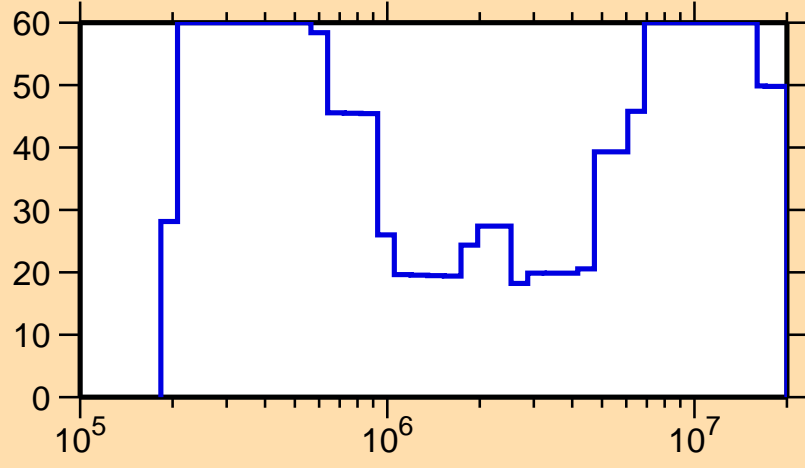
\Delta\sigma/\sigma vs. E for ^{48}\text{K}(n,\text{el.})
