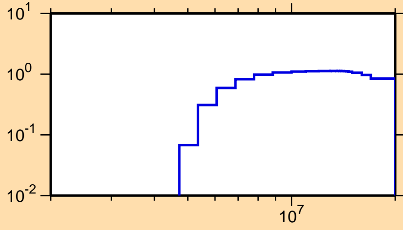
\sigma vs. E for ^{48}\text{K}(n,2n)
