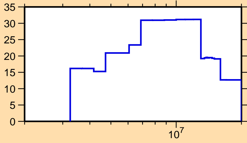
\Delta\sigma/\sigma vs. E for ^{48}\text{K}(n,\text{tot.})
