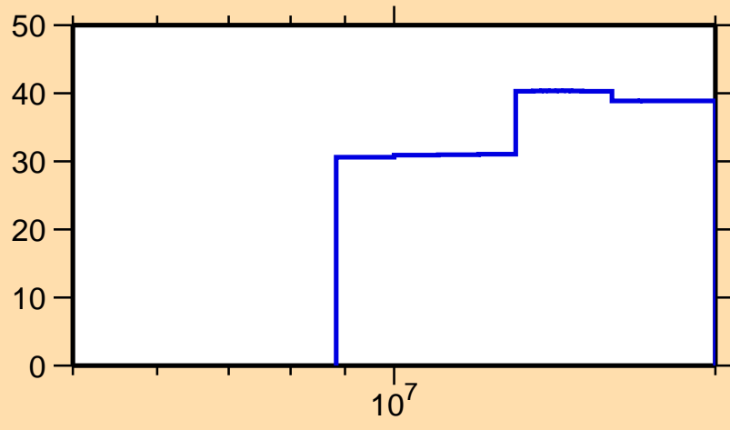
\Delta\sigma/\sigma vs. E for ^{48}\text{K}(n,n\text{cont.})
