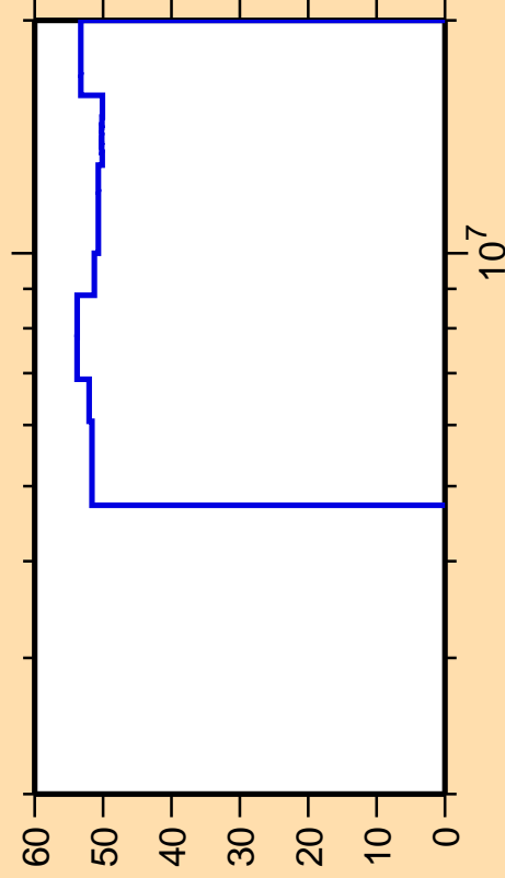
\Delta\sigma/\sigma vs. E for ^{48}\text{K}(n,2n)
