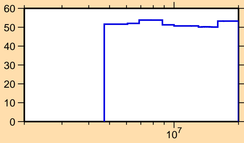
\Delta\sigma/\sigma vs. E for ^{48}\text{K}(n,2n)
