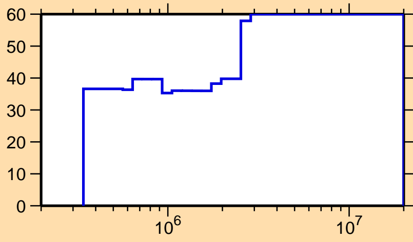
\Delta\sigma/\sigma vs. E for ^{48}\text{K}(n,n_1)
