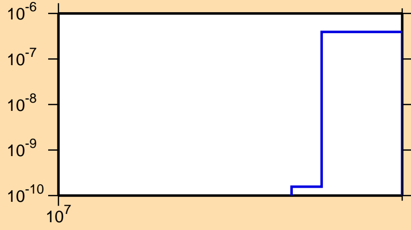
\sigma vs. E for ^{48}\text{K}(n,n\alpha)
