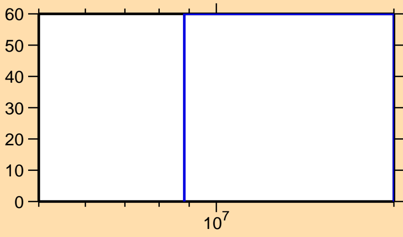
\Delta\sigma/\sigma vs. E for ^{48}\text{K}(n,\text{inel.})
