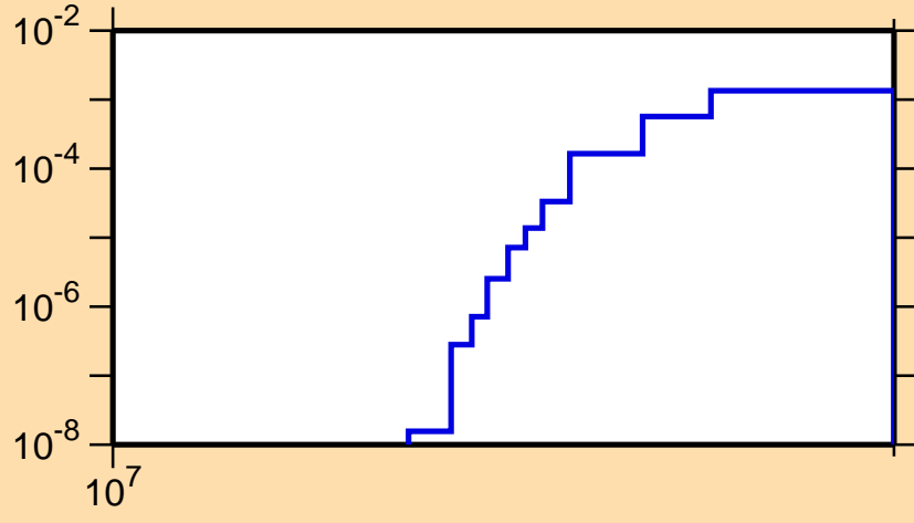
\sigma vs. E for ^{48}\text{K}(n,d)
