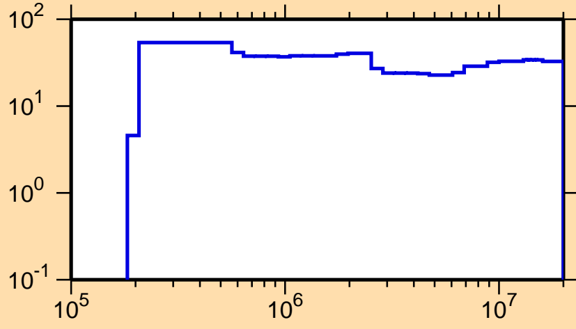
\Delta\sigma/\sigma vs. E for ^{48}\text{K}(n,\text{nonel.})
