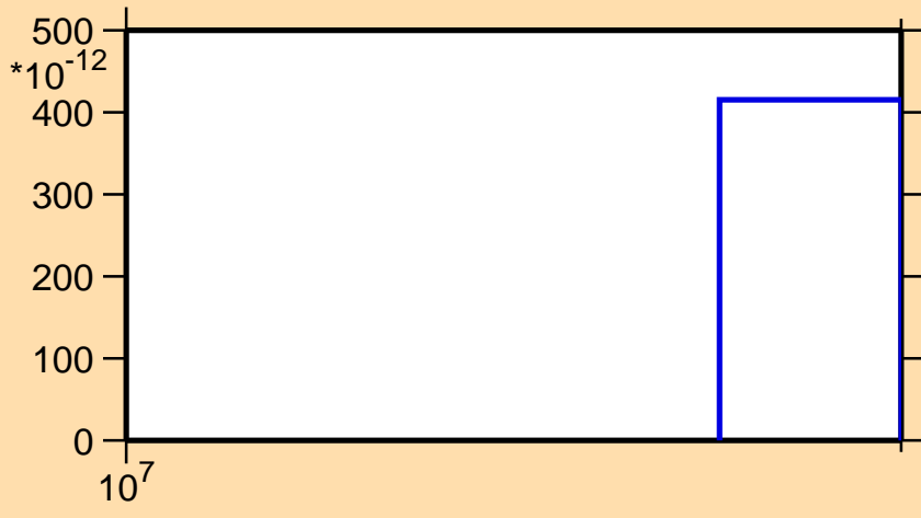
\sigma vs. E for ^{48}\text{K}(n,2np)
