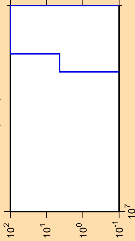
\Delta\sigma/\sigma vs. E for ^{48}\text{K}(n,nd)
