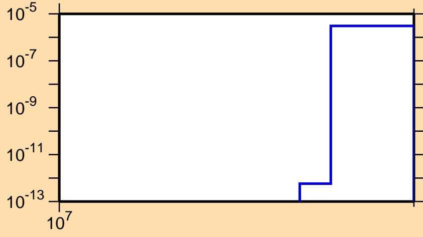
\sigma vs. E for ^{48}\text{K}(n,nd)
