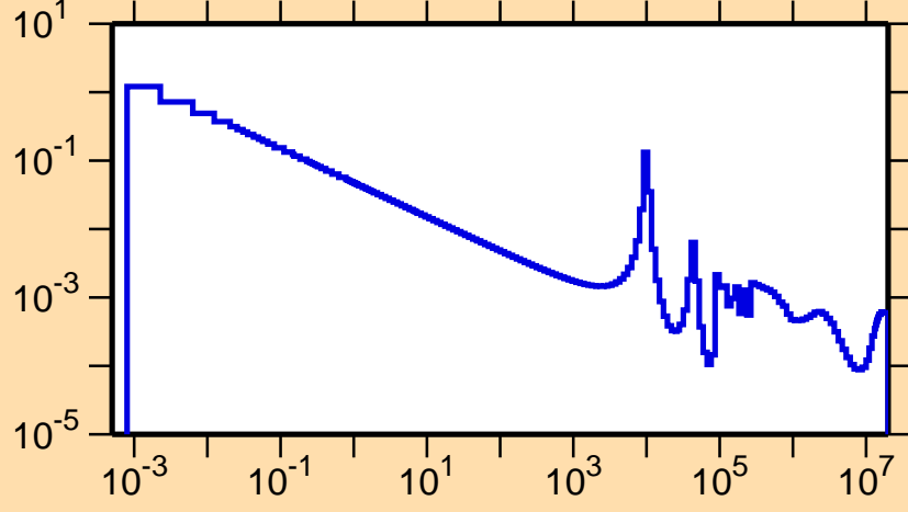
\sigma vs. E for ^{48}\text{K}(n,\gamma)
