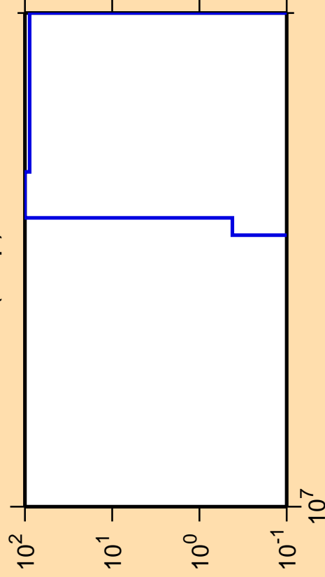
\Delta\sigma/\sigma vs. E for ^{48}\text{K}(n,np)
