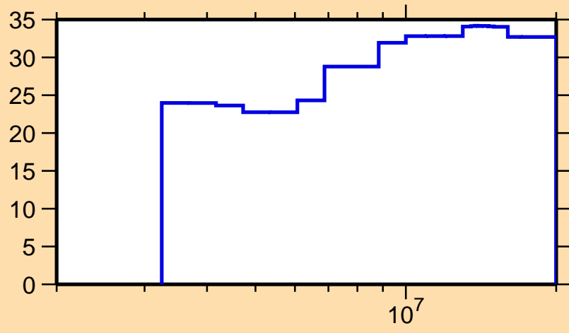
\Delta\sigma/\sigma vs. E for ^{48}\text{K}(n,n\text{onel.})
