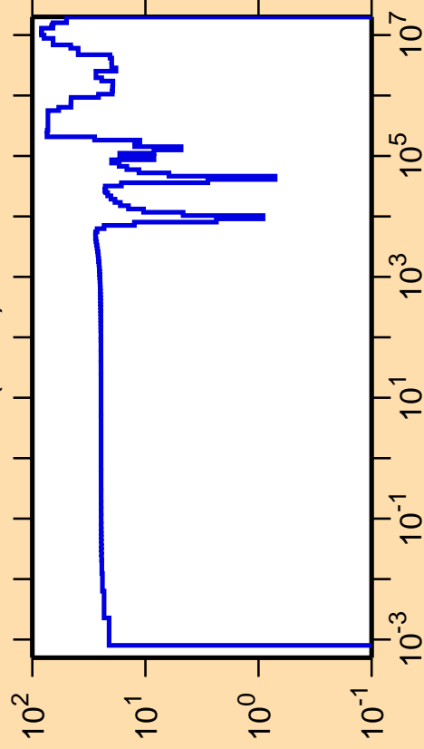
\Delta\sigma/\sigma vs. E for ^{48}\text{K}(n,\text{el.})
