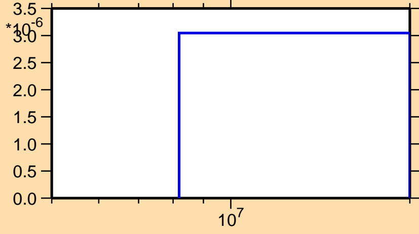
\sigma vs. E for ^{48}\text{K}(n,\alpha)
