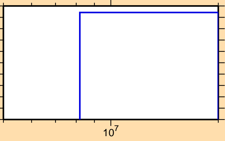
\sigma vs. E for ^{48}\text{K}(n,3n)
