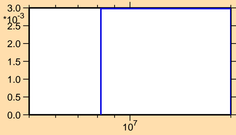
\sigma vs. E for ^{48}\text{K}(n,p)
