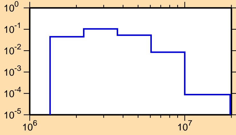
\sigma vs. E for ^{49}\text{K}(n,n_4)
