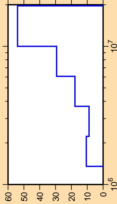
\Delta\sigma/\sigma vs. E for ^{49}\text{K}(n,n_4)
