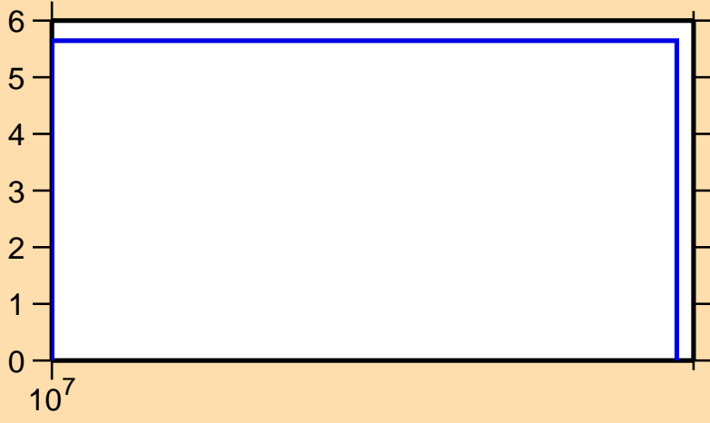
\Delta\sigma/\sigma vs. E for ^{49}\text{K}(n,\text{el.})
