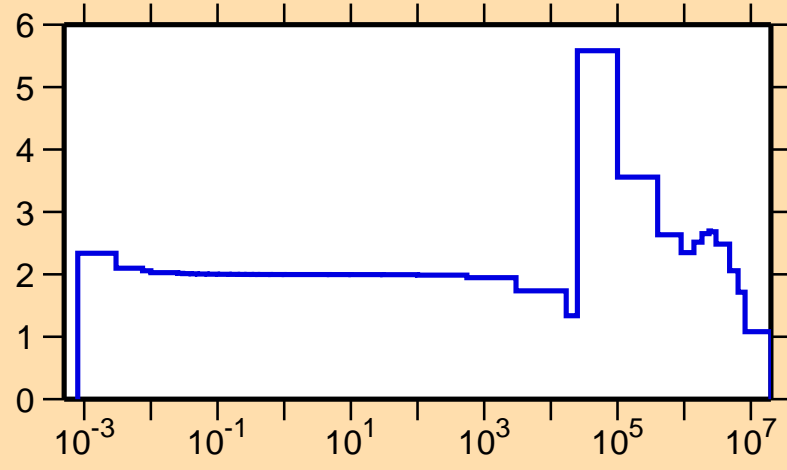
\sigma vs. E for ^{49}\text{K}(n,\text{el.})
