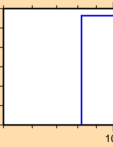
\sigma vs. E for ^{49}\text{K}(n,p)
