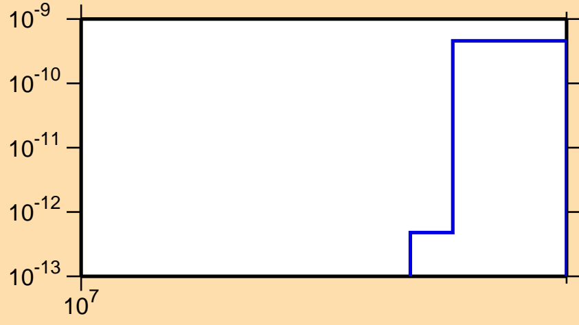
\sigma vs. E for ^{72}\text{Kr}(\text{mt } 34)
