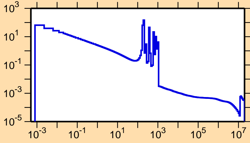
\sigma vs. E for ^{72}\text{Kr}(n,\gamma)
