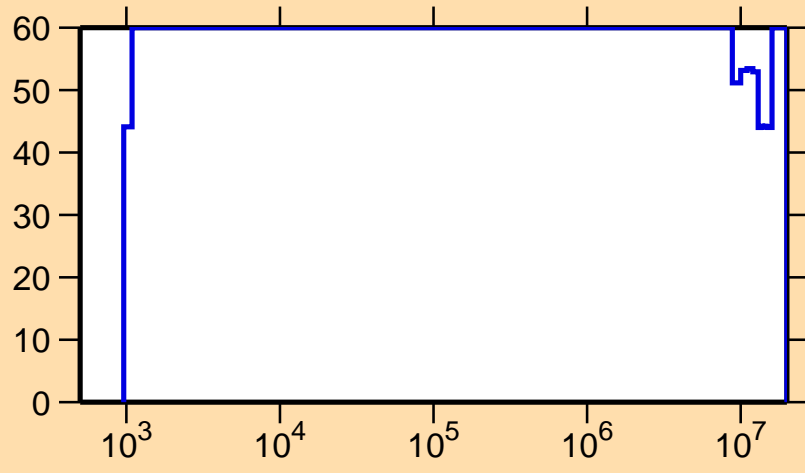
\Delta\sigma/\sigma vs. E for ^{72}\text{Kr}(n,\gamma)
