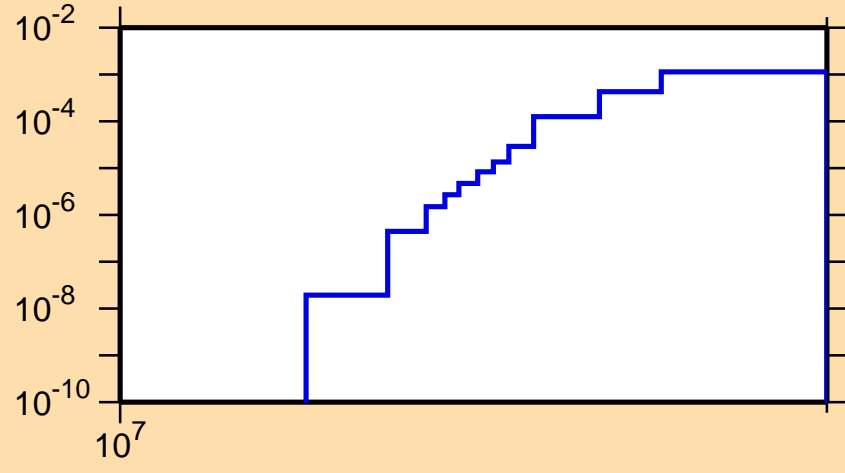
\sigma vs. E for ^{72}\text{Kr}(n,t)
