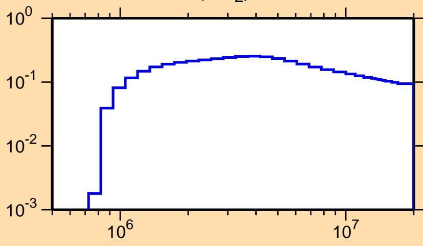
\sigma vs. E for ^{72}\text{Kr}(n,n_2)
